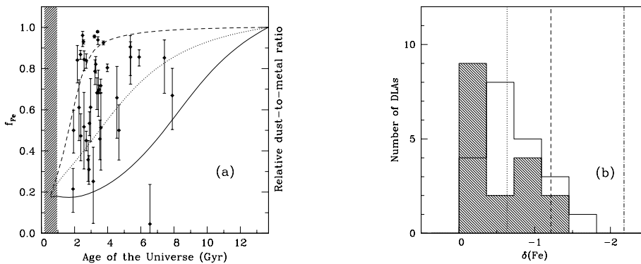
Fig. 4. Time evolution of the dust content in DLA systems. a) Diamonds: f_{\text{Fe}} versus age of the universe; dashed area: reionization epoch 6 \leq z \leq 20 (Fan et al. 2003; Spergel et al. 2003); solid, dotted and dashed curves: Inoue's (2003) model predictions of the evolution of the relative dust-to-metal ratio for different sets of input parameters (see text for explanations); the curves have been normalized to the present-day value and scaled assuming a formation redshift z_f = 20 . b) Frequency distribution of iron depletions in two bins of look-back time (shaded area: t_l \geq 10.5 Gyr; empty histogram: t_l < 10.5 Gyr). The fraction in dust are computed for the set of parameters Sa.
