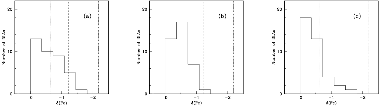
Fig. 1. Distribution of iron depletions for the DLA systems in Table 1. Panels a) , b) and c) correspond to cases Sa, Sb and E1, respectively. Vertical lines: typical values of interstellar iron depletions in the Milky Way (dotted line: warm halo gas; dashed line: warm disk gas; dotted-dashed line: cold disk gas).
