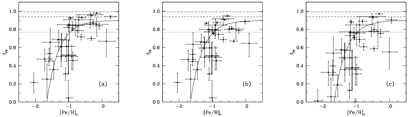
Fig. 2. Iron dust fraction versus metallicity for the sample of DLA systems listed in Table 1. Panels a) , b) and c) correspond to cases Sa, Sb and E1, respectively. Horizontal lines: representative values of iron dust fractions in the Galactic ISM (legenda as in Fig. 1). Solid curve: empirical law (4) describing the evolution of the dust fraction with metallicity.
