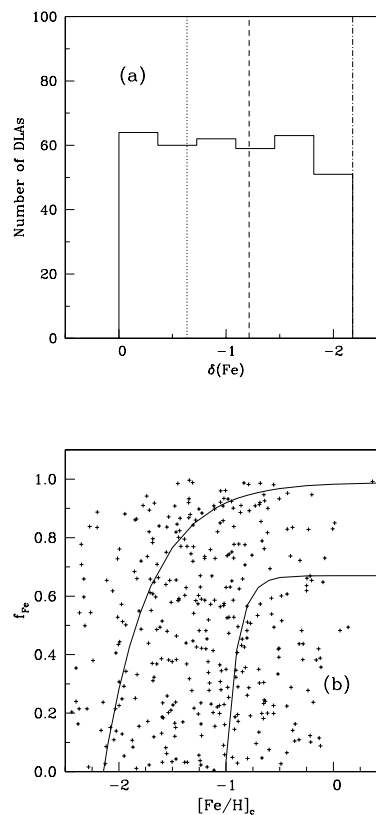
Fig. 3. Test of selection effects performed on a mock sample of n = 1000 DLA systems with H I, Fe II and Zn II column densities rejected as explained in Section 3.3. a) Frequency distribution of iron depletions resulting (after rejection) for an adopted flat distribution of \delta(\text{Fe}) . b) Dust fraction versus metallicity resulting for an adopted flat distribution of f_{\text{Fe}} ; the solid curves represent the envelopes of the real data in Fig. 2. The depletions of the mock sample have been modeled with the set of parameters Sa (Table 1); similar results are obtained for the other cases.
