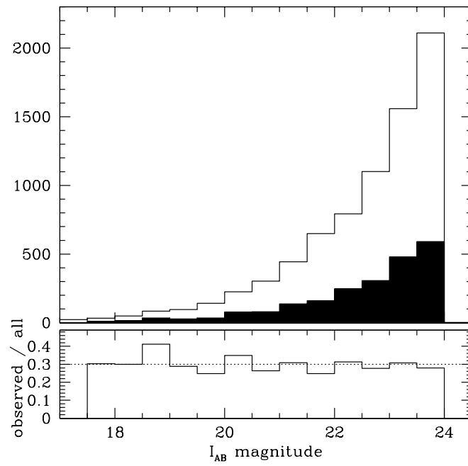
Fig. 4. (Top panel) I_{AB} magnitude distribution of objects observed with VIMOS in the Chandra Deep Field South (shaded histogram), compared to the distribution of all objects in the area in the EIS photometric catalog (open histogram). (Bottom panel) The ratio of observed vs. all objects is 0.3.
