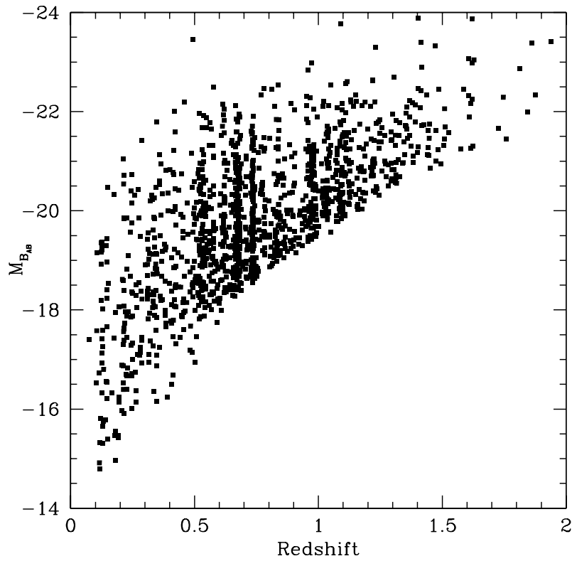
Fig. 6. Absolute M_{B_{AB}} magnitude - Redshift distribution for the full VVDS–CDFS sample
