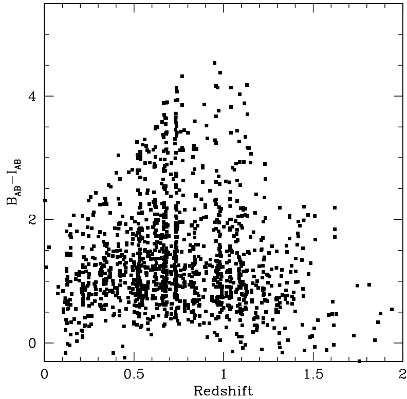
Fig. 7. B_{AB} - I_{AB} vs. Redshift distribution for the full VVDS–CDFS sample
