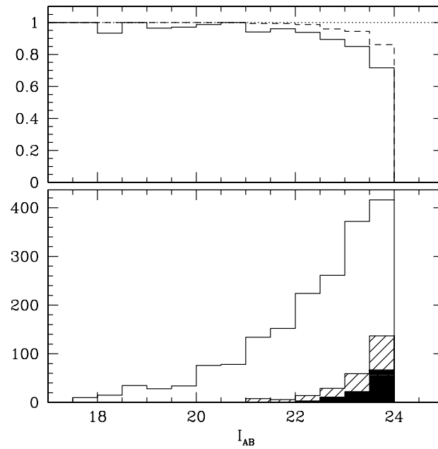
Fig. 3. Completeness of the I_{AB} \leq 24 sample. (Bottom panel) The magnitude distribution of galaxies with secure redshift measurements (flags 2,3,4,9; open histogram), uncertain and failed measurements (flags 0 and 1, dashed histogram), and failed measurements alone (flags 0, filled histogram). (Top panel) the ratio of secure redshift measurements (flags 2,3,4,9 continuous line histogram), and of all measurements (flags 1,2,3,4,9 dashed line histogram). The overall redshift measurement completeness is 88% (flags 2,3,4,9) and redshifts are measured for 95% of the sample.
