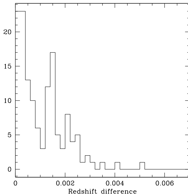
Fig. 2. Redshift difference between objects observed twice or more in independent VIMOS observations. The distribution has a velocity dispersion \sigma_z = 0.0012 or 360km/s.
