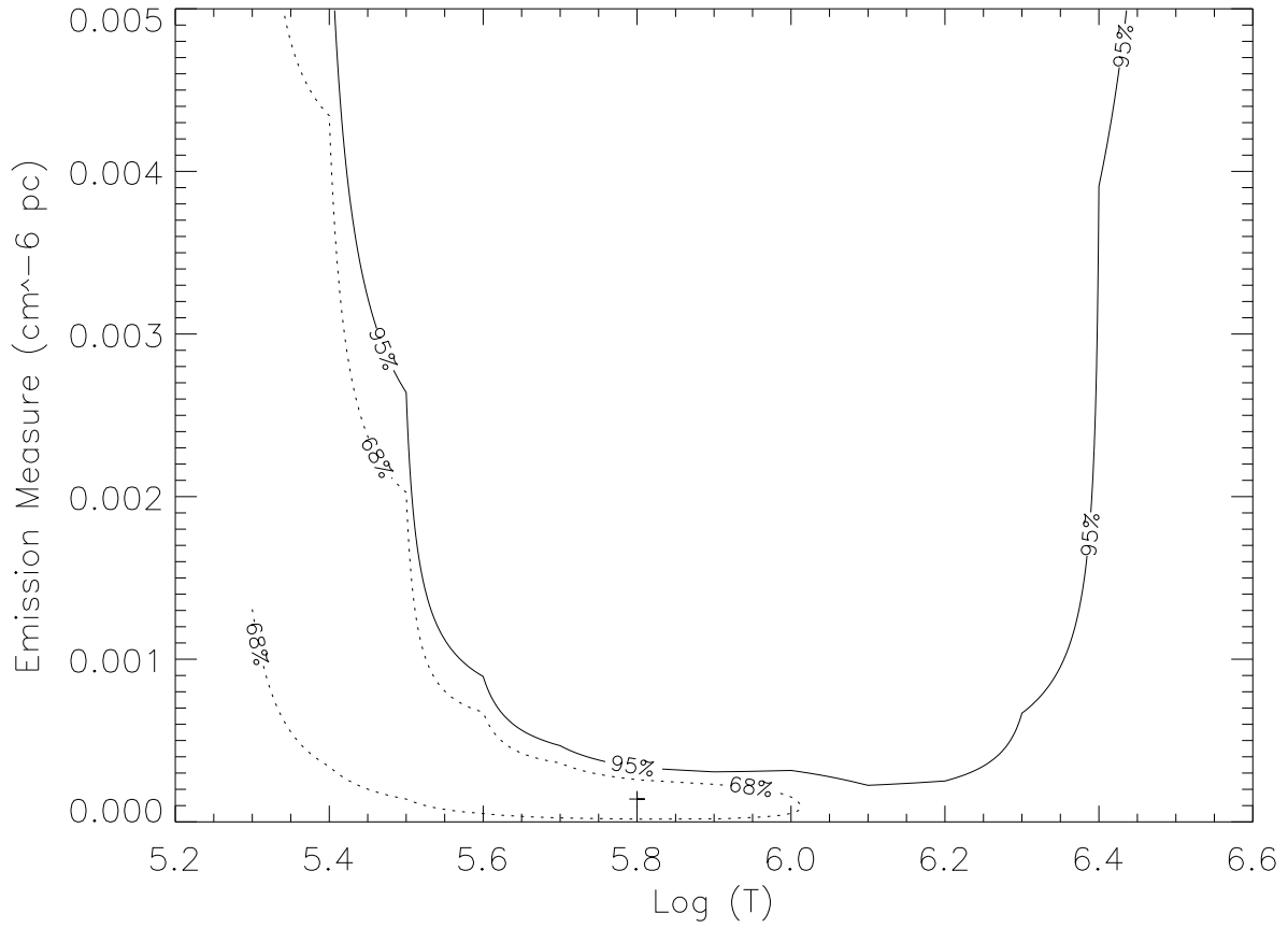
Fig. 3.— Constraints on temperature and emission measure based on CHIPS observations, and APEC/CHIANTI equilibrium ionization plasma code with solar abundances. See text for discussion.
