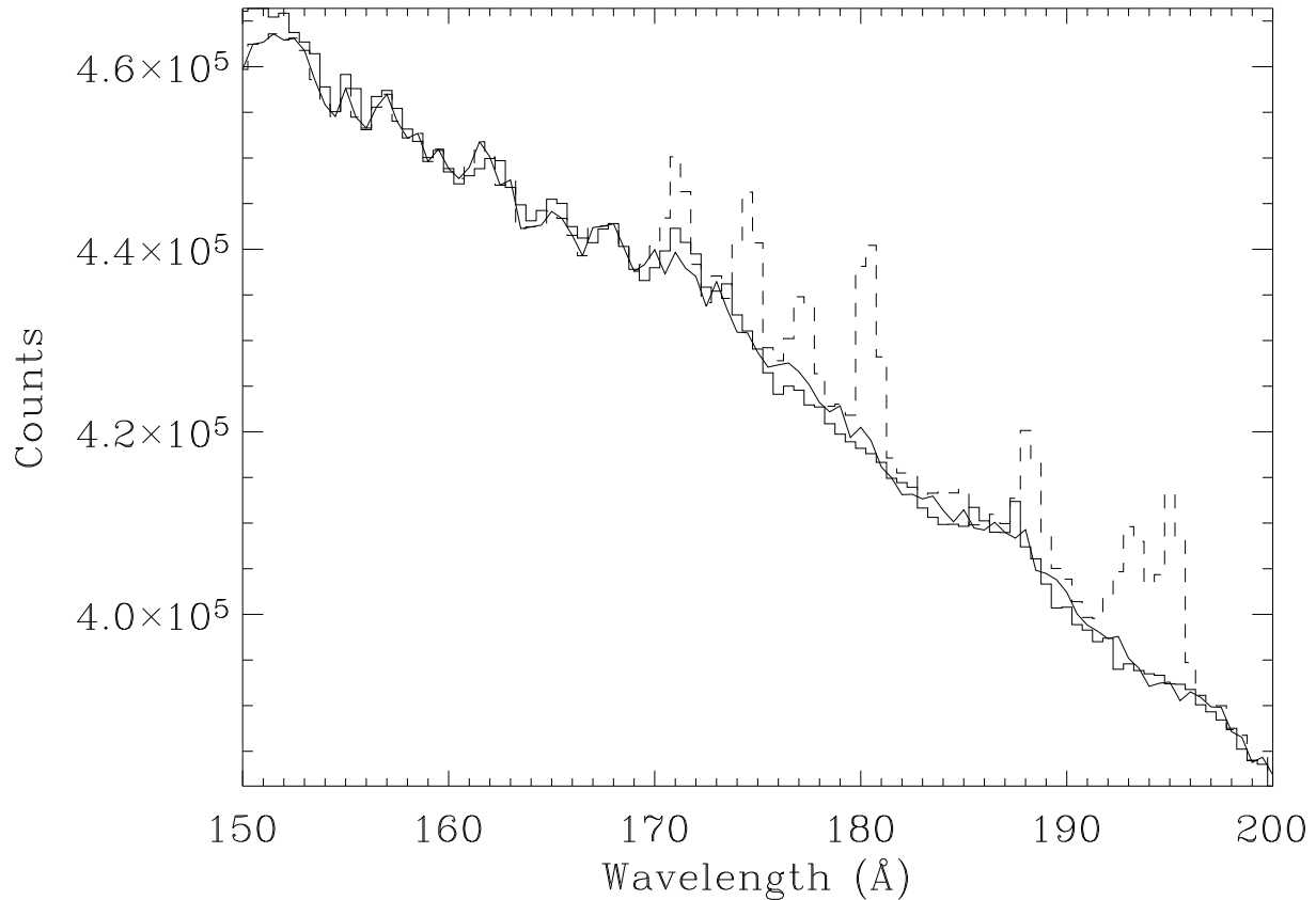
Fig. 2.— Coadded spectrum from 150 - 200 Å of all fields, summing both filter panels (solid histogram). Vertical axis shows total counts in bins of 0.5 Å. We also show a scaled, charged-particle background spectrum (solid line) and background plus predictions of "canonical" local hot bubble model with temperature of 10^{6.1} K and emission measure of 0.0038 \text{ cm}^{-6} \text{ pc} (dashed histogram), adapted to the same spectral bin size. The most significant excess observed above background is near 171 Å.
