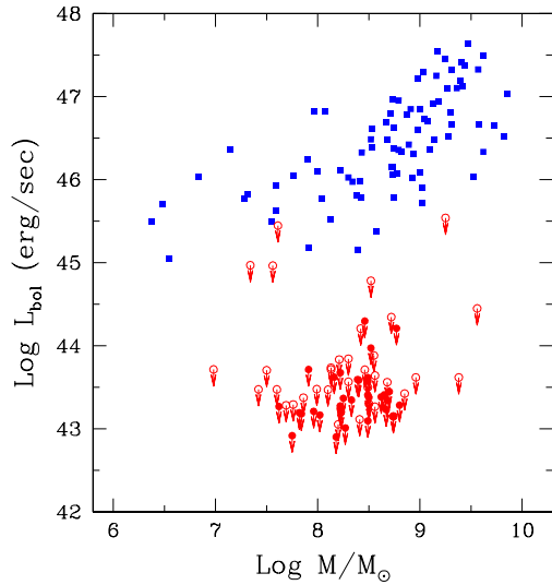
Fig. 7.— Bolometric luminosity vs. black hole mass for radio-loud AGNs. The bolometric luminosities of BL Lac objects are presented as an upper limit, after beaming correction with an averaged lower limit to the Doppler factor, \delta \gtrsim 3.9 . For the observed black hole mass range 10^7 < M_{\bullet}/M_{\odot} < 4 \times 10^9 , the bolometric luminosity spans over 4 orders of magnitude, indicating a large difference in Eddington ratio among radio-loud AGNs. Squares : radio-loud AGN from Woo & Urry (2002a); filled circles : BL Lac objects with black hole mass from the measured \sigma_e ; open circles : BL Lac objects with black hole mass from r_e and \mu_e .
