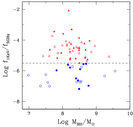
Fig. 3.— X-ray to radio flux ratio vs. black hole mass for our sample of BL Lac objects. Black hole masses are estimated from the measured \sigma_e (filled symbols) or r_e and \mu_e (open symbols). The dashed line divides high-frequency peaked BL Lac objects (triangles) [colored red in electronic edition] from low-frequency peaked objects (circles) [colored blue in electronic edition] following Perlman et al. (1996). The black hole mass spans over 2 orders of magnitude independent of BL Lac spectral type. The black hole mass estimated from \sigma_e are distributed over a narrower range because of the relatively small volume sampled ( \langle z \rangle \sim 0.17 ).
