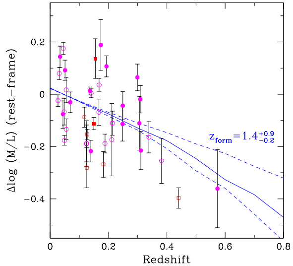
Fig. 10.— Evolution of the rest-frame mass-to-light ratio of AGN host galaxies in the Cousins R band. The mass-to-light ratio for individual galaxies are derived after K -correction with the z_{form} = 1.4 model. Circles : host galaxies of BL Lac objects; squares : radio galaxies; open symbols : galaxies with mass < 5 \times 10^{11} M_\odot ; filled symbols : galaxies with mass > 5 \times 10^{11} M_\odot ; solid line : a single burst model with z_{form} = 1.4 , which has \Delta \log(M/L)/\Delta z = -0.502 between z = 0 and z = 0.4 ; dashed lines : single burst models with z_{form} = 1.2 and 2.3 , showing the uncertainty range determined in the observed mass-to-light ratio evolution (see §4.2). The observed trend is similar to that of early-type galaxies (Treu et al. 2002; van Dokkum & Franx 2001; Treu et al. 2002).
