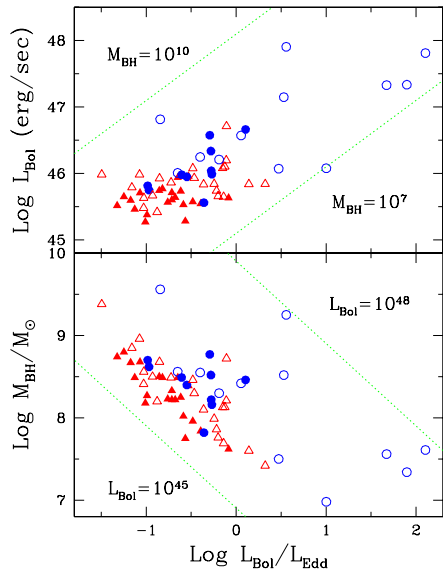
Fig. 5.— Bolometric luminosity ( top ) and black hole mass ( bottom ) vs. Eddington ratio. LBLs and HBLs are overlapping in black hole mass. However, LBLs generally have higher Eddington ratios compared with HBLs. Symbols are the same as in Figure 3. The absence of higher and lower black hole mass AGNs in the top panel as well as higher and lower luminosity AGNs in the bottom panel are likely caused by selection effects (see text).
