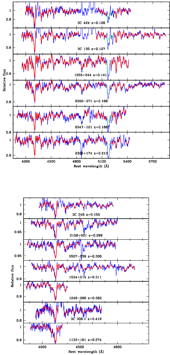
Fig. 1.— Observed spectra of AGN host galaxies ( thin line [colored blue in electronic edition]), with best-fit templates ( thick line [colored red in electronic edition]). Top panels : Spectra of six galaxies with large wavelength coverage. Bad pixels, AGN emission lines, and the Mgb triplet lines ( dotted line [colored green in electronic edition]) were masked out before fitting. Bottom panel : Seven galaxies with smaller fitting ranges.
