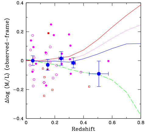
Fig. 8.— Evolution of the observed-frame mass-to-light ratio of AGN host galaxies in the Cousins R band. The evolution of the mass-to-light ratio is consistent with single burst models with z_{form} = 1.4^{+0.9}_{-0.2} within the 68% confidence level. \Delta \log(M/L) is defined as the difference in logarithm between the M/L at each redshift and the M/L in our lowest AGN host redshift bin ( z = 0.046 ). Large filled circles : averaged \Delta \log(M/L) for each redshift bin with 1 \sigma error bars; small circles : individual host galaxies of BL Lac objects; squares : individual radio galaxies; small open symbols : individual host galaxies with mass less than 5 \times 10^{11} M_{\odot} ; small filled symbols : individual host galaxies with mass greater than 5 \times 10^{11} M_{\odot} ; dashed line : stellar population synthesis model with single burst at z_{form} = 1 ; solid line : a single burst model with z_{form} = 1.5 ; dotted line : a single burst model with z_{form} = 2 ; thin-solid line : a single burst model with z_{form} = 5 . For clarity no error bars are shown on the measurements for individual galaxies. For these the reader is referred to Figure 10, which shows the same measurements with error bars, albeit in the rest-frame rather than the observed frame.
