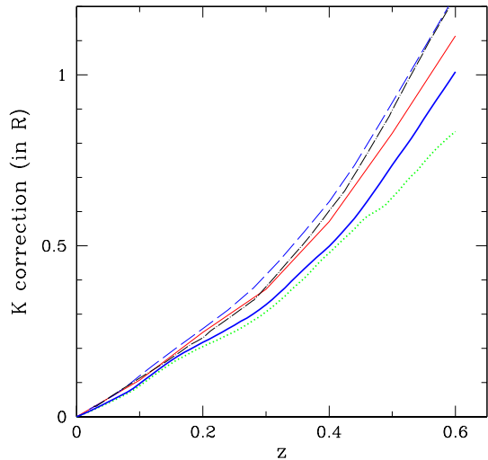
Fig. 9.— K -correction values for different stellar population synthesis models. Dotted line : a single burst at z = 1 ; solid line : a single burst at z = 1.4 ; thin-solid line : a single burst at z = 5 with a cosmology with \Omega = 0.3 , \Lambda = 0.7 , and H_o = 70 \text{ km sec}^{-1} \text{ Mpc}^{-1} . Dashed line : K -correction values from Poggianti 1997, where a cosmology with q_o = 0.225 , H_o = 50 \text{ km sec}^{-1} \text{ Mpc}^{-1} was used. Dot-dashed line : K -correction values from Fukugita et al. 1995, based on the observed spectra of nearby galaxies with no stellar population evolution using a cosmology with q_o = 0 and H_o = 50 \text{ km sec}^{-1} \text{ Mpc}^{-1} .
