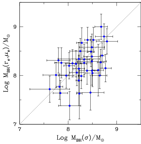
Fig. 2.— Comparison of black hole mass estimates of 32 BL Lac objects from the stellar velocity dispersions (Table 3) and from r_e and \mu_e using the Coma cluster fundamental plane relation, converted for a cosmology with H_o = 70 \text{ km s}^{-1} \text{ Mpc}^{-1} , \Omega = 0.3 , \Lambda = 0.7 . The surface brightness \log I is corrected for the rest-frame Cousins R -band luminosity evolution of stellar populations using d \log L / d \log z = 0.502 (see §4.3). The measurement errors of r_e , \mu_e , and \sigma are considered in the error propagation. The intrinsic scatter in the fundamental plane (0.08 in \log r_e ) is also included in the error estimation of black hole mass from r_e and \mu_e (Woo et al. 2004). The rms scatter between two black hole mass estimates is 0.34 dex.
