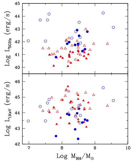
Fig. 4.— Radio and X-ray luminosity vs. black hole mass. Neither X-ray nor radio luminosity is correlated with black hole mass. LBLs tend to have higher radio and lower X-ray luminosity for a given black hole mass. Symbols are the same as in Figure 3.
