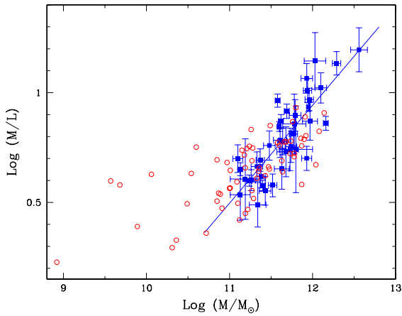
Fig. 11.— Galaxy mass-to-light ratio vs. galaxy mass. The mass-to-light ratios for our AGN host galaxies ( filled squares ), corrected for luminosity evolution using a z_{form} = 1.4 model, are compared with those of nearby elliptical galaxies ( open circles ) from van der Marel & van Dokkum (2005). The mass-to-light ratios in the Cousins R band for the nearby galaxies were calculated using B - R = 1.57 . The solid line corresponds to the best fit to the AGN host galaxies. The mass-to-light ratio vs. mass relation of the AGN host galaxies is consistent with that of normal galaxies in the mass range where the data sets overlap ( 11 < \log M/M_{\odot} < 12 ).
