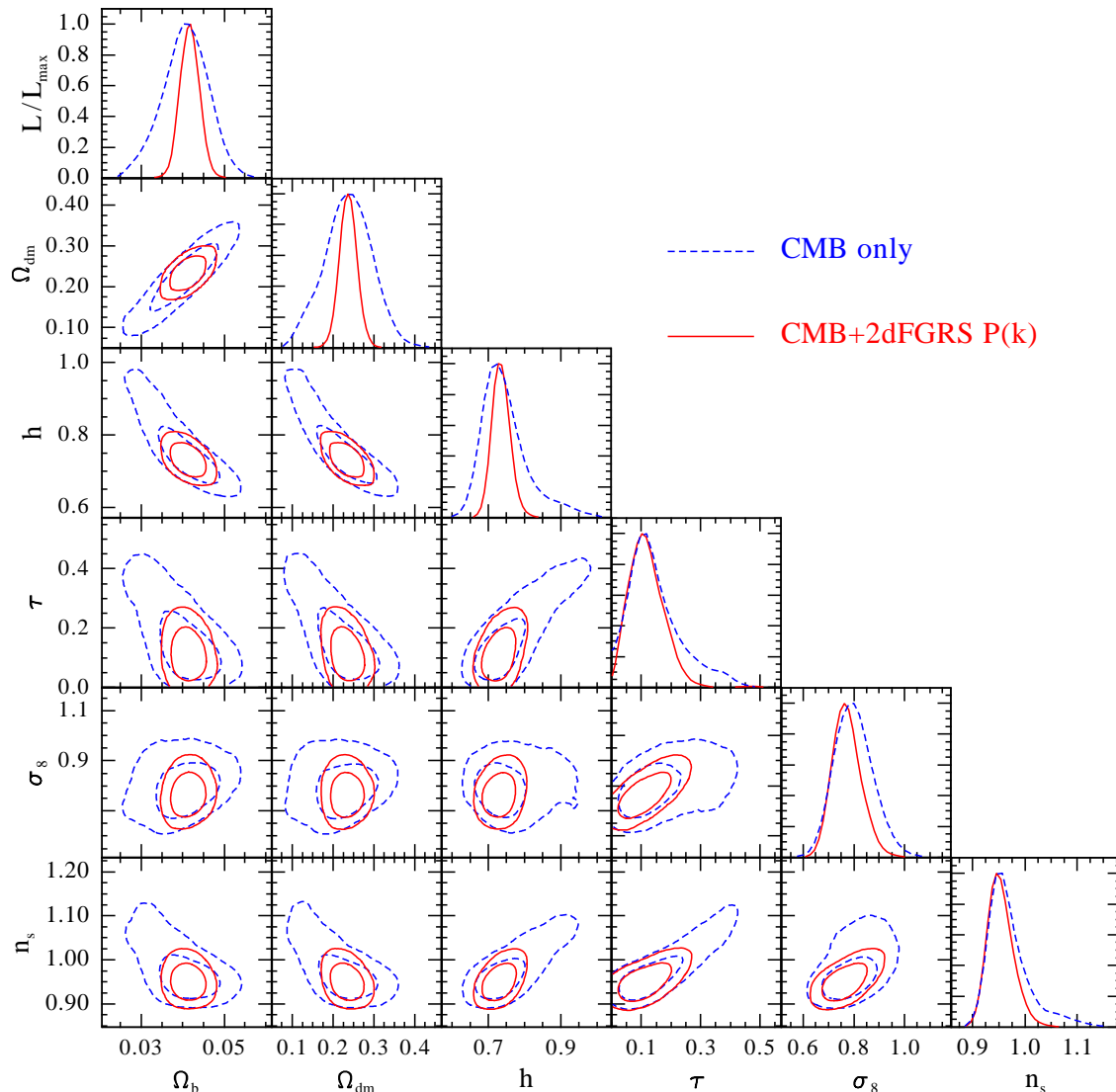
Figure 2. Marginalized posterior likelihoods for the cosmological parameters in the basic-six model determined from CMB information only (dashed lines) and CMB plus 2dFGRS P(k) (solid lines).
