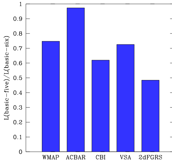
Figure 17. The likelihood ratios of the basic-five model to the basic-six model plotted in Fig.16 for the individual datasets used in our analysis.
