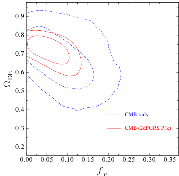
Figure 4. The marginalized posterior likelihood in the f_\nu - \Omega_{\text{DE}} plane for the basic-six+ f_\nu parameter set. The dashed lines show the 68% and 95% contours obtained in the CMB only case. The solid contours show the parameter constraints obtained for combined CMB and 2dFGRS P(k) datasets.
