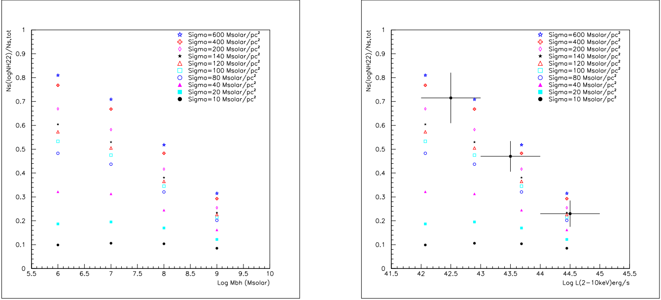
Fig. 4. Expected behaviour of the fraction N_s(\log N_H > 22)/N_{s,tot} , for several values of \Sigma , as a function M_{BH} (left hand panel) and of L(2-10 \text{ keV}) (right hand panel), with the latter derived assuming L_{bol}/L_{Edd}=0.1 (e.g. Peterson et al. 2004) and the luminosity–dependent bolometric correction in Marconi et al. (2004). In the right hand panel, crosses represent the observed fraction (corrected for selection effects, and adapted from La Franca et al. 2005) of obscured AGN in the local universe.
