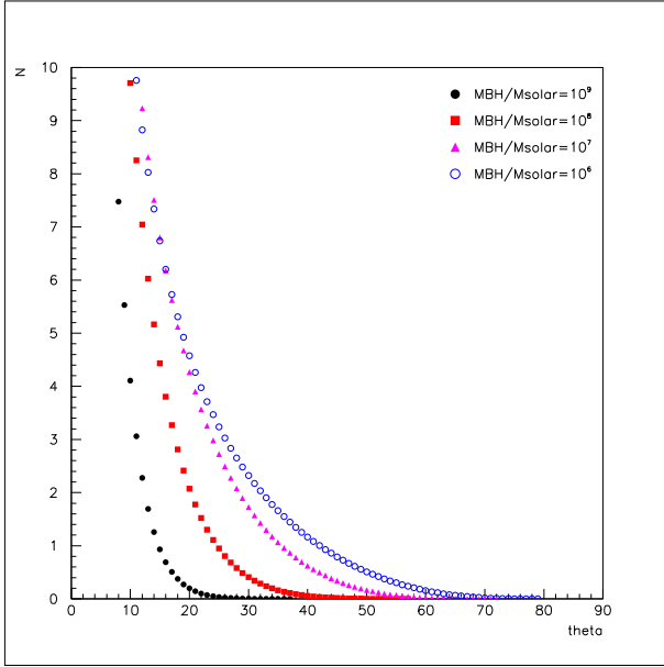
Fig. 3. Number of clouds along the line of sight as a function of \theta for four values of M_{BH} , when \Sigma = 200 M_\odot \text{pc}^{-2}
