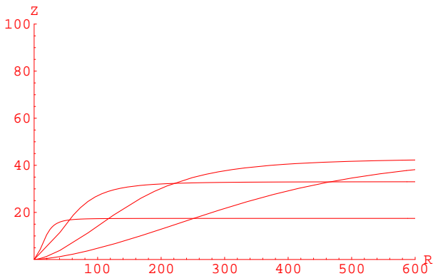
Fig. 2. Scale height of the clouds as a function of R when M_{BH}=10^6 M_\odot , 10^7 M_\odot , 10^8 M_\odot and 10^9 M_\odot .
