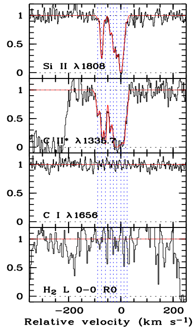
Fig. 3. Absorption line profiles of the C II* \lambda 1335 doublet and the Si II \lambda 1808 transition. Nine individual components were needed to perform the fit to the absorption lines that is overplotted to the data as a solid line. The components are indicated by vertical dashed lines. The portions of the spectrum where the C I \lambda 1656 and H 2 L 0-0 R0 transitions are expected are also shown. The zero point of the velocity scale has been taken at z_{\text{abs}} = 2.03954 .
