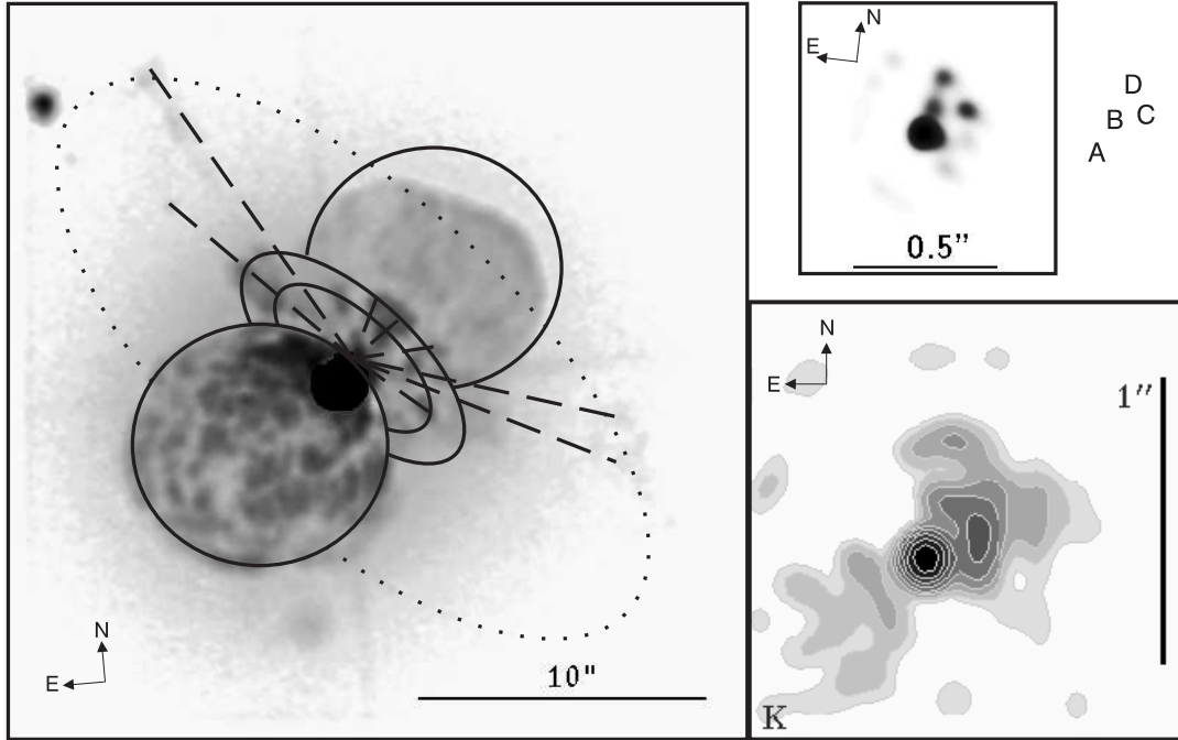
Fig. 2. — Left panel: Same as Fig. 1; broken lines indicating some of the streamers in the equatorial plane; full ellipses indicating the locations of knots in the streamers with similar radial distances from the central object; additionally the two large Homunculus outflows are indicated. Right panels: central arcseconds with the speckle objects; upper panel: 850 nm (from Hofmann & Weigelt 1993); object A is the central object itself, while objects B, C, and D are the speckle objects; lower panel: K-band image (from Rigaut, this volume). The scale in left panel is ten times that of both right panels. The exact directions North are indicated in the individual panels.
