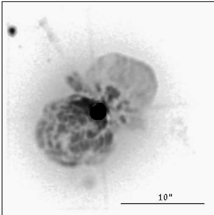
Fig. 1. — Long-exposure image of \eta Carinae obtained by averaging 200 re-centered short exposures. For details see Sect. 2.
