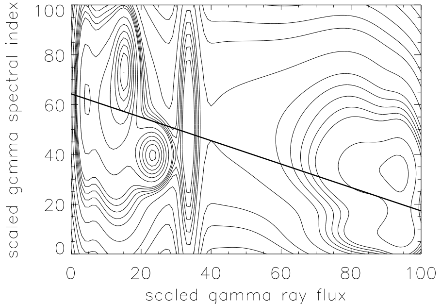
Figure 4. Scaled \gamma -ray spectral index (0=hardest occurrence minus 1\sigma , 100=softest occurrence plus 1\sigma ) in comparison to the \gamma -ray flux. Here the data are represented by ellipsoidal Gaussians and the fit is based on \chi^2 statistic.
