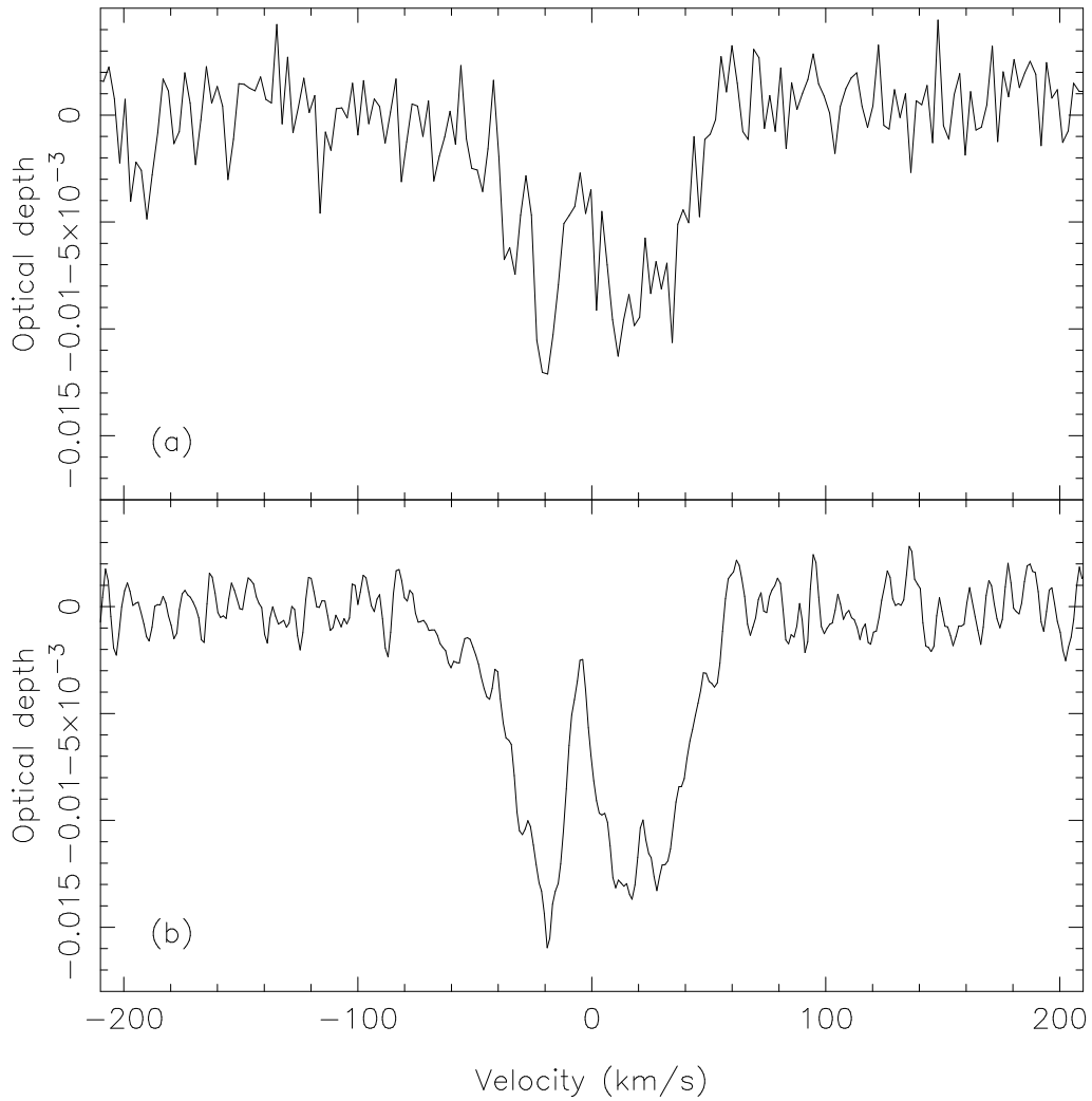
Fig. 1.— a) Discovery spectrum taken at Parkes with the Project Phoenix SETI Receiver. b) Confirmation spectrum taken with the ATCA during our VLBI observations. The velocity scale on the horizontal axis assumes HI as the molecular species.
