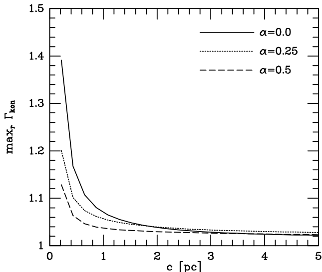
Figure 14. The maximum of \Gamma_{\text{konus}} over radius r for our cusped ‘konus’-density \rho_c (7.6) as function of its scalelength c , and cusp slope \alpha . Increasing the cusp slope, decreases the mass fraction added to the center by the ‘konus’-density, therewith resulting in a smaller dynamical effect as compared to that of the BH.
