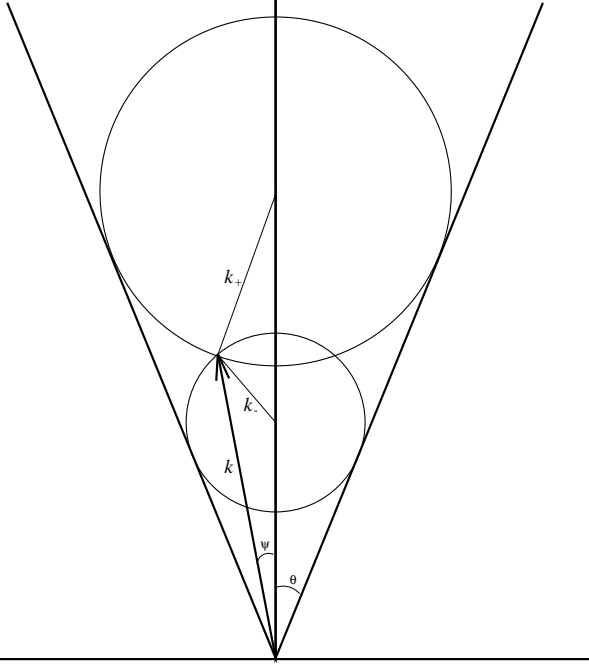
Figure 16. The build-up of the Fourier Transform H(k, \psi) of the semi-konus density inside a cone with half-angle \theta , by a weighted sum of spheres. At each point (k, \psi) with \psi < \theta there are two spheres with radii k_+ and k_- that contribute to H(k, \psi) .
