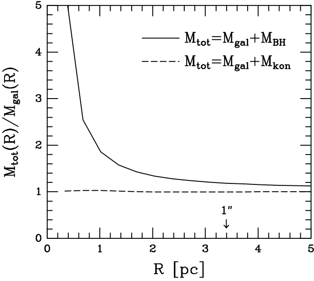
Figure 12. The total mass inside a sphere of radius R , M_{\text{tot}}(R) , over the mass of the M32 density model inside the same sphere as function of radius R . The solid line shows the case in which the total mass is build up of the (\alpha, \beta, \gamma) -model of M32 with in addition a BH of 1.8 \times 10^6 M_{\odot} . The dashed line is for the case in which we have added the maximum generalized konus density with b = 1.0'' to the density model of M32.
