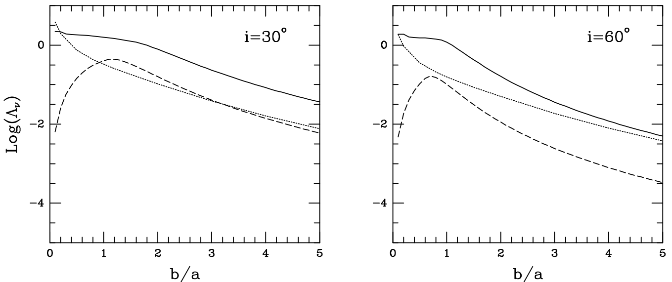
Figure 6. The maximum amount of konus density \Lambda_\nu that can be added to a perfect oblate spheroid with q = 0.8 , as determined from three different criteria: \rho > 0 (solid lines), \partial\rho/\partial\nu < 0 (dashed lines), and the empirical criterion that the minor axis surface brightness profile should not have wiggles (dotted lines). The results are shown as function of b/a for two different inclination angles ( i = 30^\circ , and 60^\circ ).
