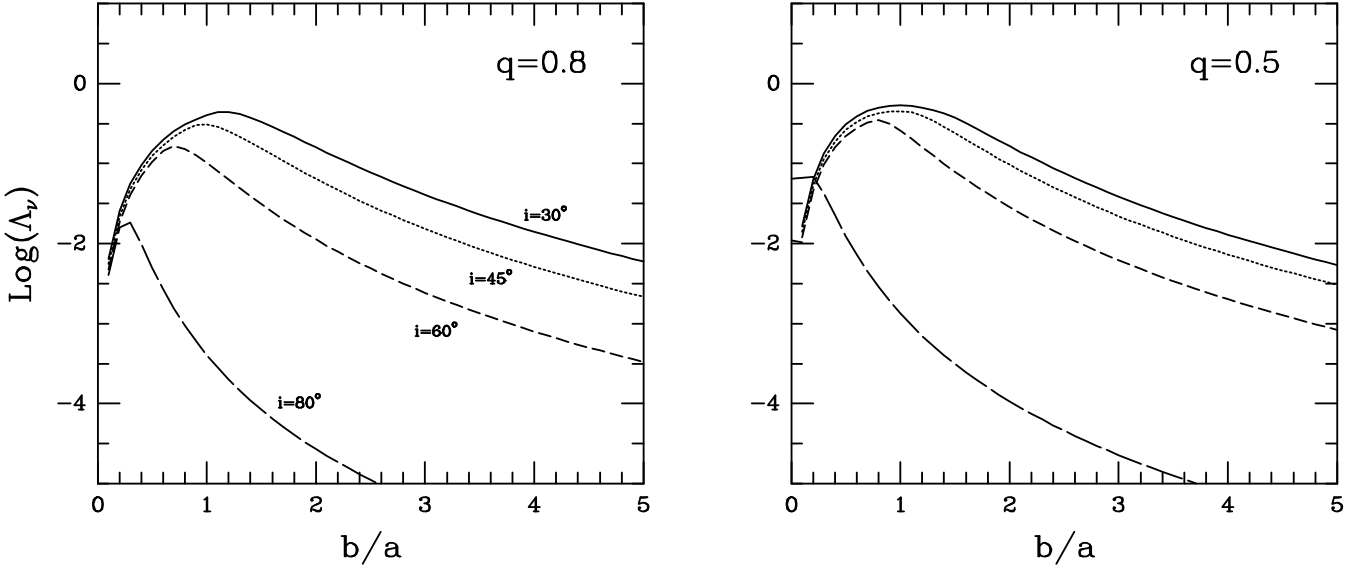
Figure 3. The logarithm of the parameter \Lambda_\nu as a function of the ratio b/a for the 6 th order generalized konus density ( \mu = 1 ). The results are presented for four different inclination angles: i = 30^\circ (solid lines), i = 45^\circ (dotted lines), i = 60^\circ (short dashed lines), and i = 80^\circ (long dashed lines). The panel on the left is for a perfect oblate spheroid with an ellipticity \epsilon of 0.2, whereas the results in the panel on the right are for a model with \epsilon = 0.5 .
