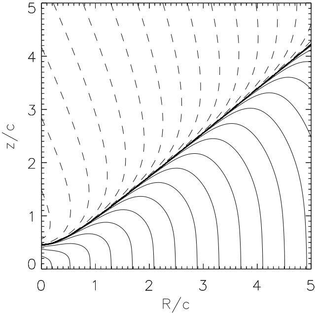
Figure 13. A contour plot of the cusped ‘konus’-density \rho_c(R, z|50^\circ) for \alpha = 0.25 . The parameters b and d are taken such that \rho_c(R, z|50^\circ) obeys the criteria (7.7) and (7.8).
