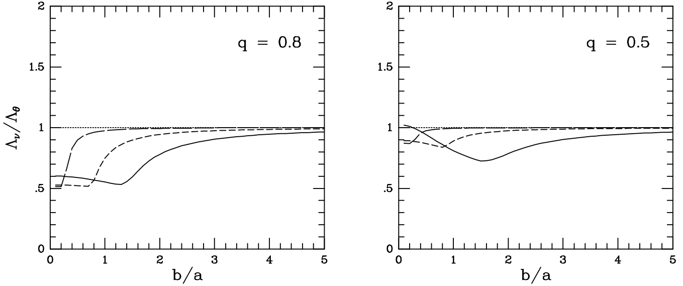
Figure 7. The ratio \Lambda_\nu/\Lambda_\theta as function of the ratio b/a of the 6 th order generalized konus density ( \mu = 1 ). The results are presented for three different inclination angles: i = 30^\circ (solid lines), i = 60^\circ (short dashed lines), and i = 80^\circ (long dashed lines). The panel on the left is for a perfect oblate spheroid with an ellipticity of 0.2, whereas the results in the panel on the right are for a model with \epsilon = 0.5 .
