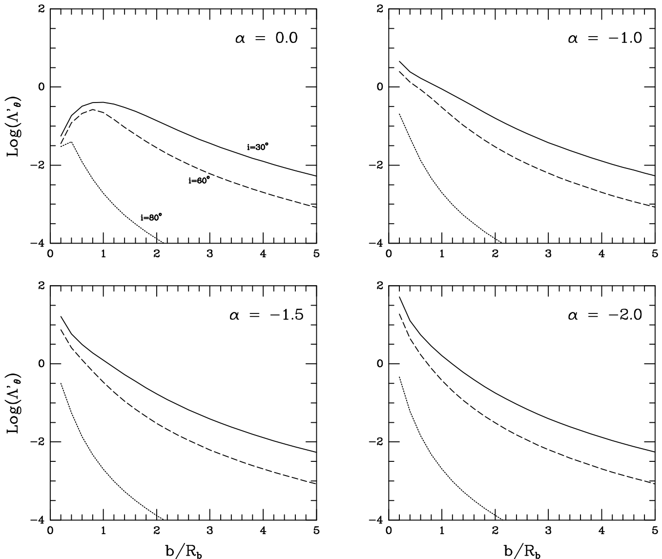
Figure 8. The ratio \Lambda'_\theta of the central density of the maximum konus density over the density of the (\alpha, \beta) -model at its core-radius R_b as function of the ratio b/R_b . Results are plotted for four different values of the cusp steepness \alpha , and for three different inclination angles: i = 30^\circ (solid lines), i = 60^\circ (dashed lines), and i = 80^\circ (dotted lines). The maximum konus density increases strongly with increasing cusp steepness and decreasing konus-scalelength b .
