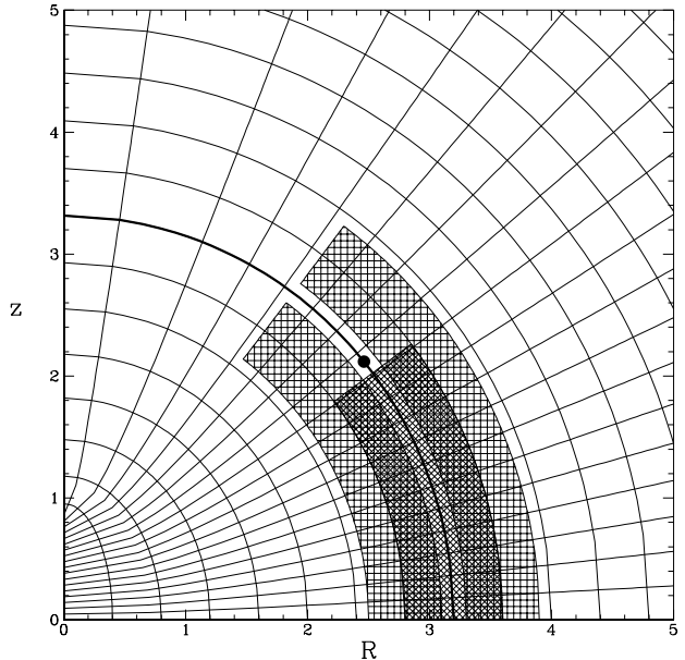
Figure 1. The grid are curves of constant \zeta and \phi , which are the curves in between which orbits in an axisymmetric potential are enclosed. The dashed regions are three such orbits. The thick, solid curve is the curve with \zeta = \zeta_0 and the solid dot is the point (\zeta_0, \phi_0) (see text). As can be seen, having zero density in (\zeta_0, \phi_0) results in zero density along the entire curve \zeta = \zeta_0 with \phi > \phi_0 .
