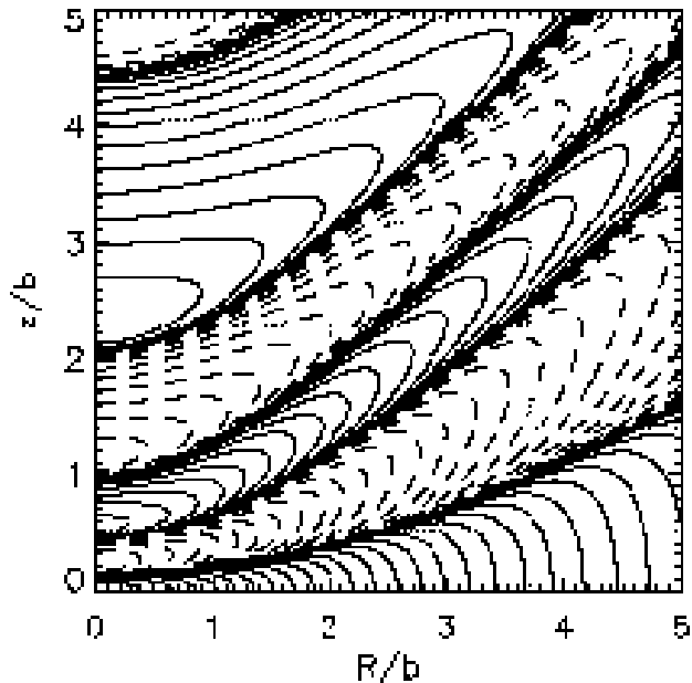
Figure 2. Contours of the 6 th order generalized konus density \rho_k^6(R, z|45^\circ) for \mu = 1 . This density distribution projects to zero surface brightness for i \leq 45^\circ . Positive contours are solid, negative contours are dashed.
