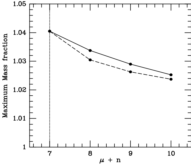
Figure 11. The maximum mass fraction \Gamma_{\max} (equation 7.4) as function of \mu + n . Since \mu \geq 1 and n \geq 6 we have a minimum \mu + n = 7 . The solid line shows \Gamma_{\text{kon}} for increasing order n ( \mu = 1 ), whereas the influence of increasing \mu (with n = 6 ) is indicated by the dashed line.
