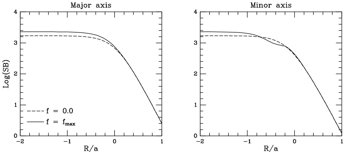
Figure 5. The luminosity profiles along the major and the minor axis of a perfect oblate spheroid with intrinsic flattening q = 0.8 seen edge-on (dashed lines). In addition, we also plot the luminosity profile of the same spheroid but to which we have added the maximum konus density \rho_k^6(R, z|30^\circ) . The scalelength of the konus density b = 1.3a , where a is the break radius of the spheroid. We have plotted the logarithm of the projected surface brightness (in arbitrary units) vs. the logarithm of the radius on the sky R in units of a .
