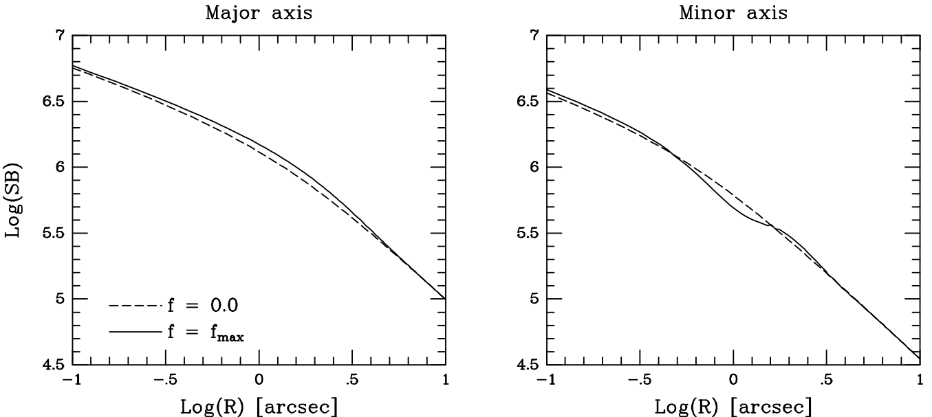
Figure 10. The logarithm of the edge-on projected surface brightness (in arbitrary units) of the (\alpha, \beta, \gamma) -model of M32, both with (solid lines) and without (dashed lines) the maximum konus density ( \mu = 1 , n = 6 ) derived from the approximate criterion.
