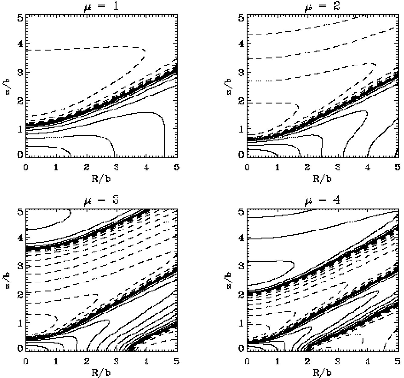
Figure 15. Contours of the generalized \rho_k(R, z|60^\circ) for \mu = 1, 2, 3, and 4 . Each of these density distributions projects to zero surface brightness for i < 60^\circ . Positive contours are solid, negative contours are dashed.
