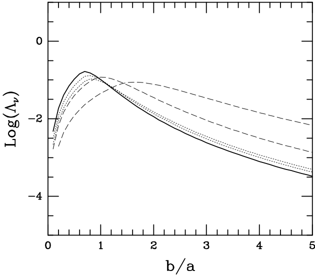
Figure 4. The same as Figure 3, except that we now plot the maximum konus densities for different orders n of the generalized konus density and for different values of \mu . All lines are for an oblate spheroid with \epsilon = 0.2 , seen under an inclination angle of 60^\circ . The thick, solid line is for \mu = 1 and n = 6 . The dashed lines are for \mu = 2 and \mu = 4 , and the dotted lines are for higher order; n = 7 and n = 8 . As can be seen, central density of the maximum konus density increases with both \mu and n for large scalelengths b . However, for small scalelengths ( b/a \lesssim 1 ), \Lambda_\nu is highest for \mu = 1 , n = 6 .
