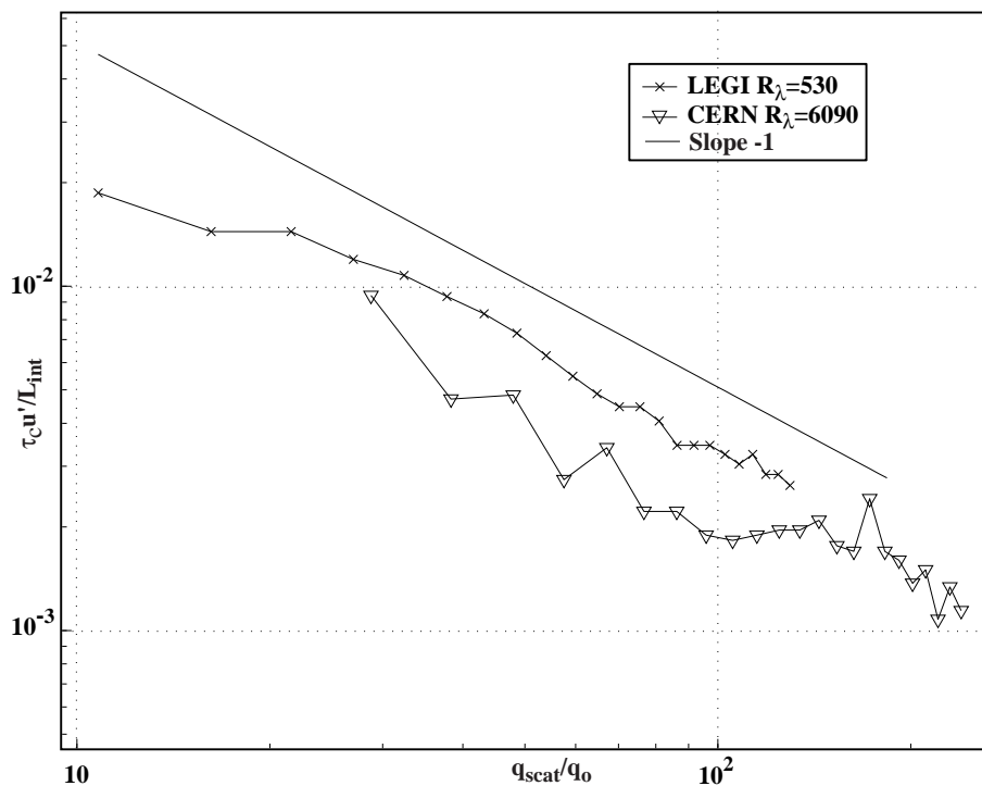
Figure 11. Scaling of \tau_s (normalized by the large scale time \tau_0 ) with the wave number q_{scat} : ( \times ) R_\lambda \simeq 530 , ( \nabla ) R_\lambda \simeq 6090 .
