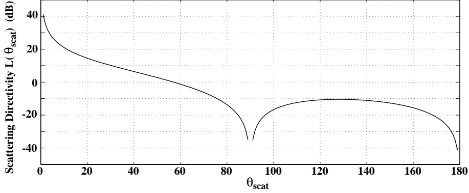
Figure 2. Acoustic Scattering by Vorticity Directivity
