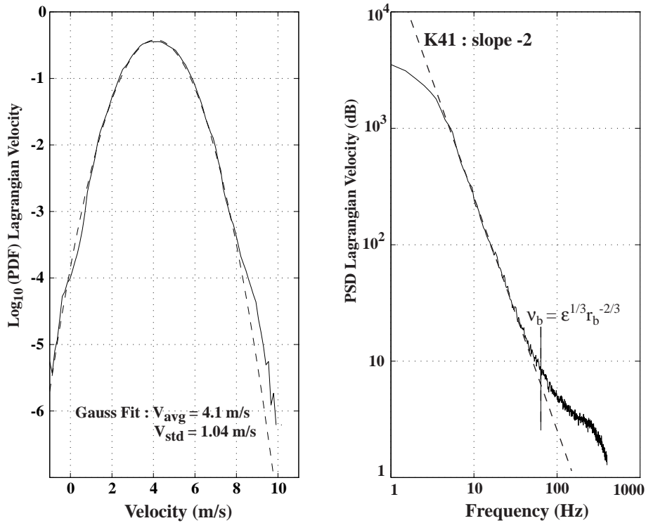
Figure 14. PDF (left) and PSD (right) of the Lagrangian Velocity in the LEGI turbulent jet flow at R_\lambda \simeq 500
