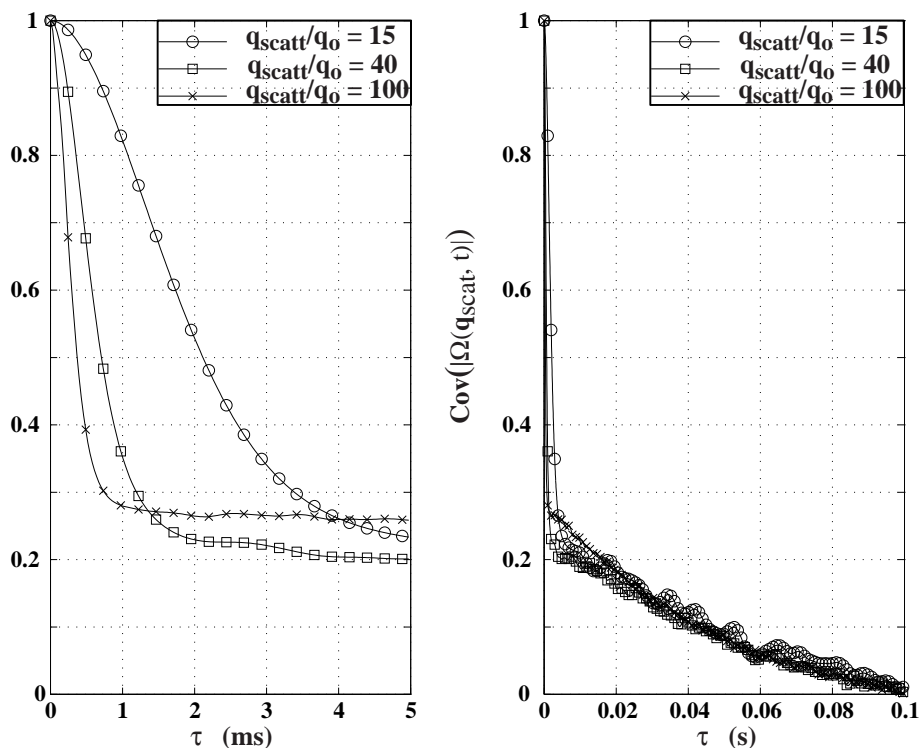
Figure 10. Time correlation of vorticity modulus for different scales 1/q_{scat} in the LEGI jet ( R_\lambda \simeq 740 ) (log-lin coordinates in the insert)
