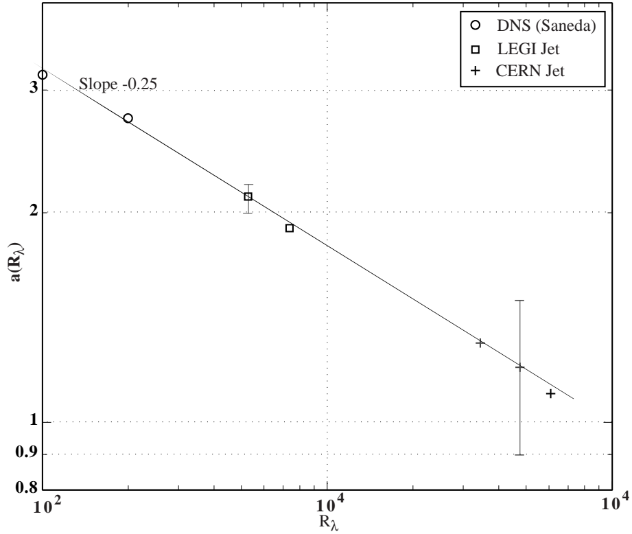
Figure 12. Power law behaviour of a(R_\lambda) in jets for 530 \leq R_\lambda \leq 6090
