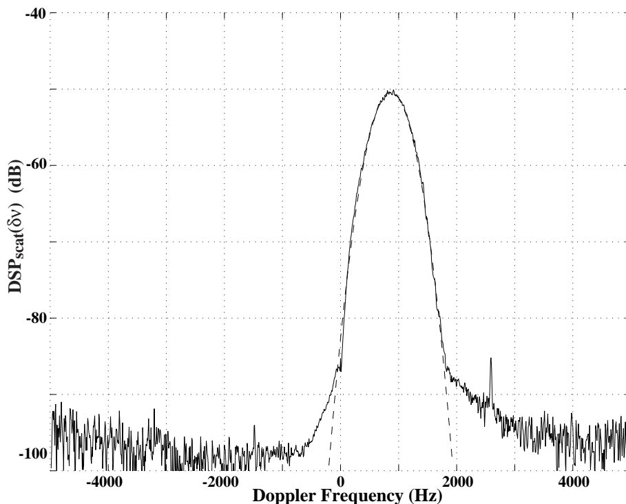
Figure 5. Power Spectral Density of \Omega_{\perp}(\mathbf{q}_{scat}, t) at a scale \sim \lambda in the LEGI jet ( R_{\lambda} \simeq 785 )
