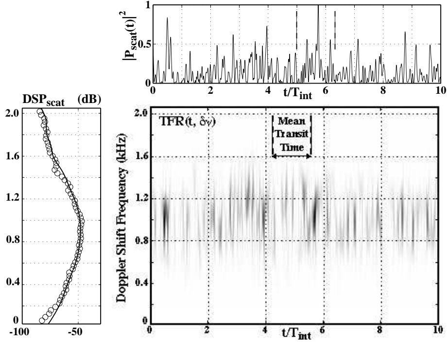
Figure 9. Time-Frequency Analysis of z_{scat}(t) in the LEGI air jet flow ( R_\lambda \simeq 785 ). Center : TFD_z(t, \nu) , Left : PSD marginal (o) and averaged PSD (-), Top : instantaneous power marginal
