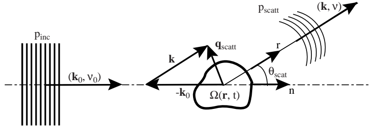
Figure 1. Acoustic Scattering by a Vorticity Distribution
