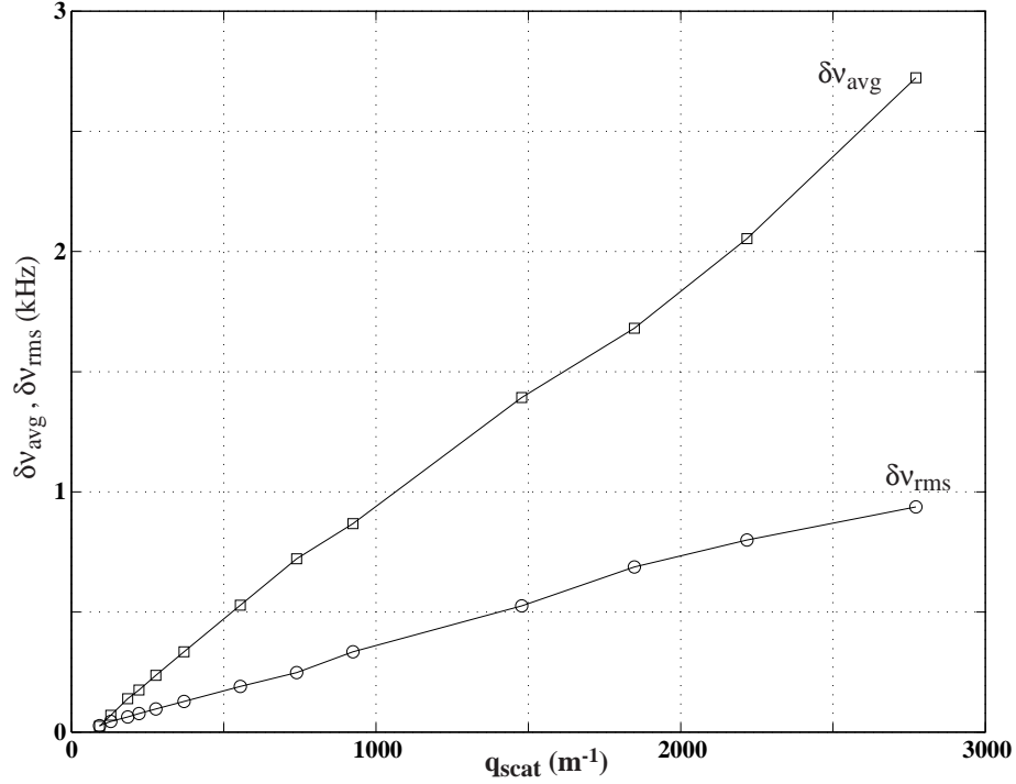
Figure 7. Evolution of the mean \delta\nu_{avg} and of the variance \delta\nu_{rms} of the Doppler shifts, with the scattering wave-number q_{scat} in the LEGI jet ( R_\lambda \simeq 785 )
