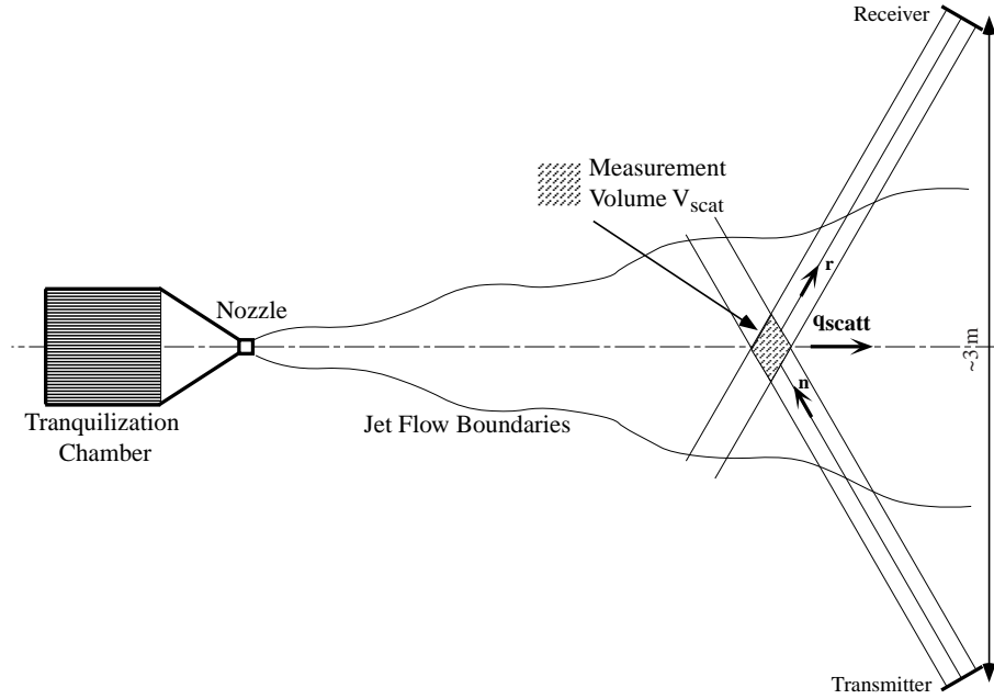
Figure 3. Acoustic scattering experiment in a turbulent jet flow
