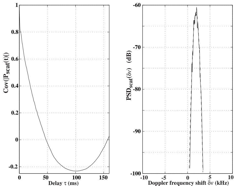
Figure 13. Normalized Covariance C_{\rho\rho}(\tau) of \rho_{scat}(t) (left) and PSD_{scat}(\delta\nu) (right) of the acoustic pressure scattered by soap bubbles in the LEGI turbulent jet flow at R_\lambda \simeq 500 .
