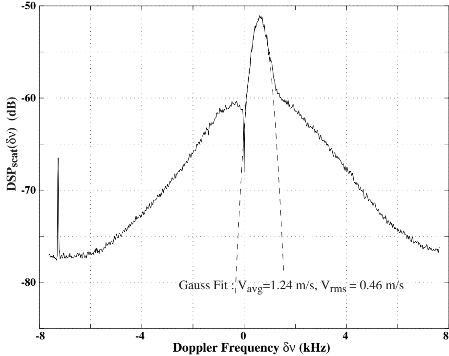
Figure 6. Power Spectral Density of \Omega_{\perp}(\mathbf{q}_{scat}, t) , at a scale \sim 3\lambda in the CERN helium jet flow ( R_{\lambda} \simeq 3450 ).
