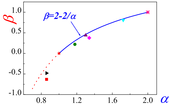
FIG. 1. The \alpha - \beta plot. Normal diffusion : \star represents models with a normal diffusion and a normal heat conduction, i.e. \alpha = 1 and \beta = 0 , such as the Lorentz gas channel[12], the Frenkel-Kontorova model[5], the \phi^4 model[9], the disordered FPU model[10], the disordered Ehrenfest gas channel[15], the irrational triangle channel[16], the alternative mass hard-core potential model[17], and some rational polygonal channel[25] etc. Ballistic motion : \ast represents the ballistic transport, i.e. \alpha = 2 and \beta = 1 , such as the 1D harmonic lattice model. Superdiffusion : \nabla , 1D Ehrenfest gas channel with right angle triangle scatterers[15]; \circ , 1D channel with rational triangle scatterers[16]; \triangle , polygonal billiard channel with one irrational ( (\sqrt{5} - 1)\pi/4 ) and one rational ( \pi/3 ) triangle; \diamond , a 1D triangle-square channel[26]. Subdiffusion : the polygonal billiard channel with one irrational angle ( (\sqrt{5} - 1)\pi/4 ) and one rational angle ( \pi/4 )[25], \square , from the channel length 1 \leq L \leq 40 ; \triangleright , from the channel of length 40 \leq L \leq 80 .
