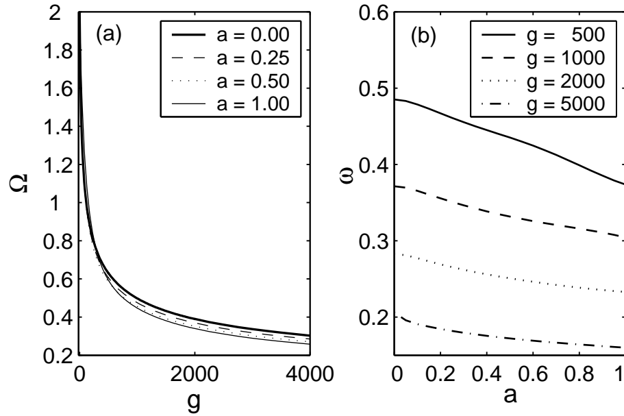
Figure 1. The threshold rotation frequency above which the 1-vortex has lower energy (in the rotating frame) than the nonvortex state vs. the strength of interaction for various values of the interaction range, panel (a), and the frequency of the anomalous mode (for \Omega = 0 ) of the 1-vortex vs. the interaction range for various values of the interaction strength, panel (b).
