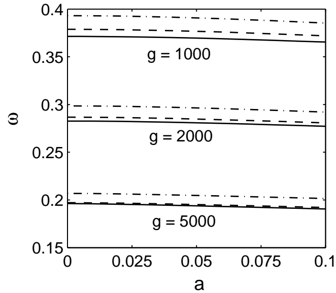
Figure 2. The frequency of the anomalous mode (for \Omega = 0 ) of the 1-vortex vs. the interaction range for various values of the interaction strength for the perturbed harmonic trap (the parabolic potential perturbed by the quartic term), the dash and dash-dot lines. The solid line corresponds to the harmonic trap.
