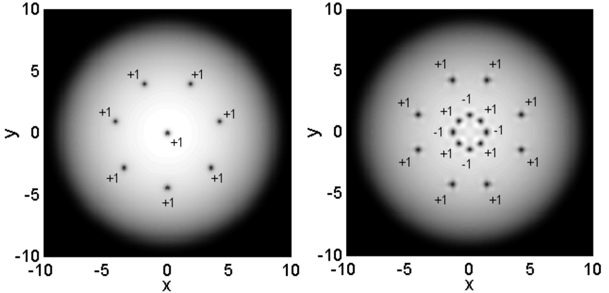
Figure 8. The stationary vortex solutions for a = 0.052 , g = 10^4 and \Omega = 0.5 . The left panel shows the 8-vortex solution and the right one – the 16-vortex solution comprised of 12 vortices and 4 antivortices.
