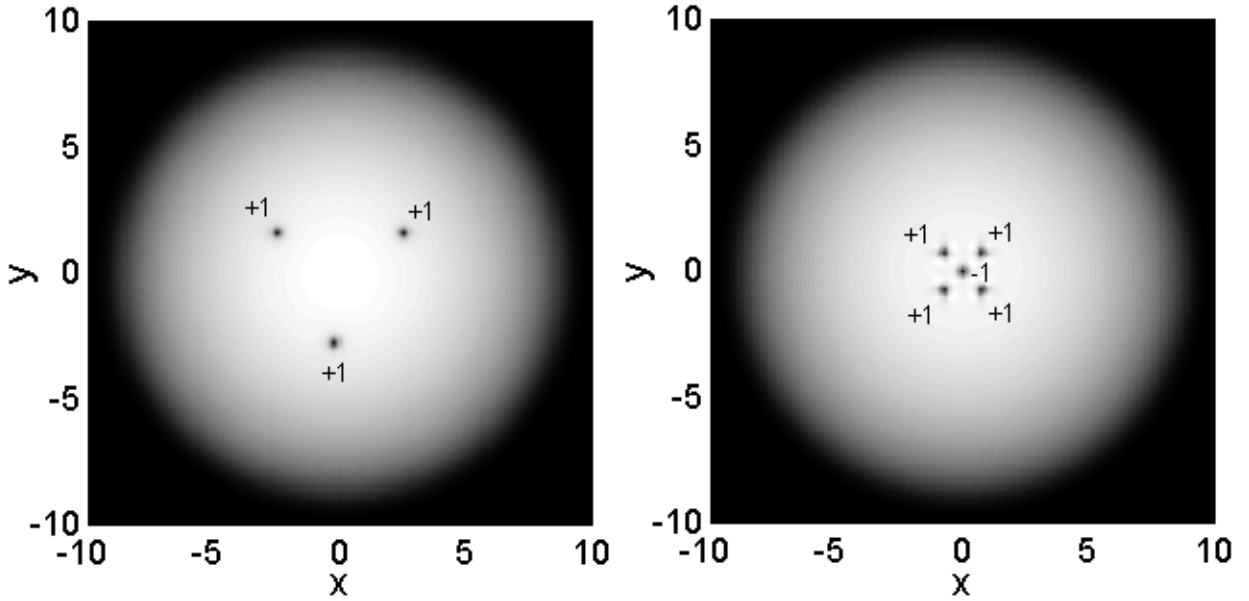
Figure 7. The stationary vortex solutions for a = 0.052 , g = 10^4 and \Omega = 0.38 . The left panel shows the 3-vortex solution and the right one – the 5-vortex solution comprised of 4 vortices and 1 antivortex (in the center).
