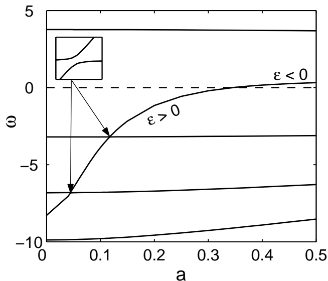
Figure 5. Zero crossing with creation of an anomalous mode with the orbital number l = 3 of the axial 2-vortex. In the picture g = 5000 and \Omega = 0 . The insert indicates the avoided crossing collisions of the normal modes.
