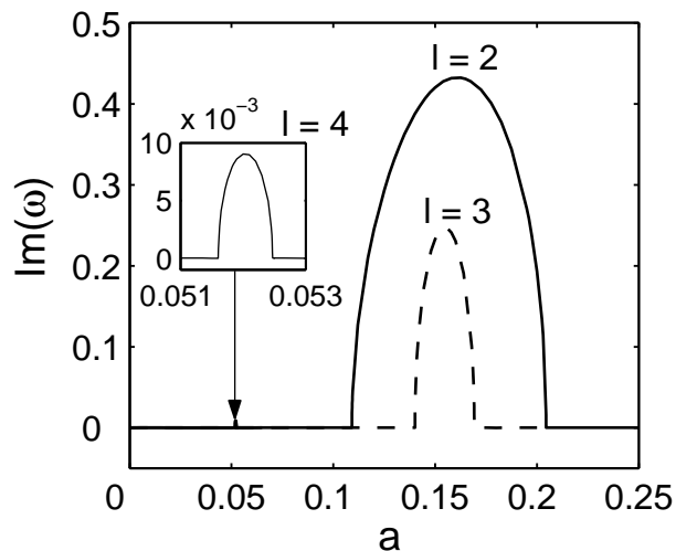
Figure 6. The imaginary part of the eigenfrequencies corresponding to the unstable orbital modes with the orbital numbers l = 2, 3 and l = 4 (in the insert) of the axial 3-vortex. Here the interaction strength is g = 10^4 .
