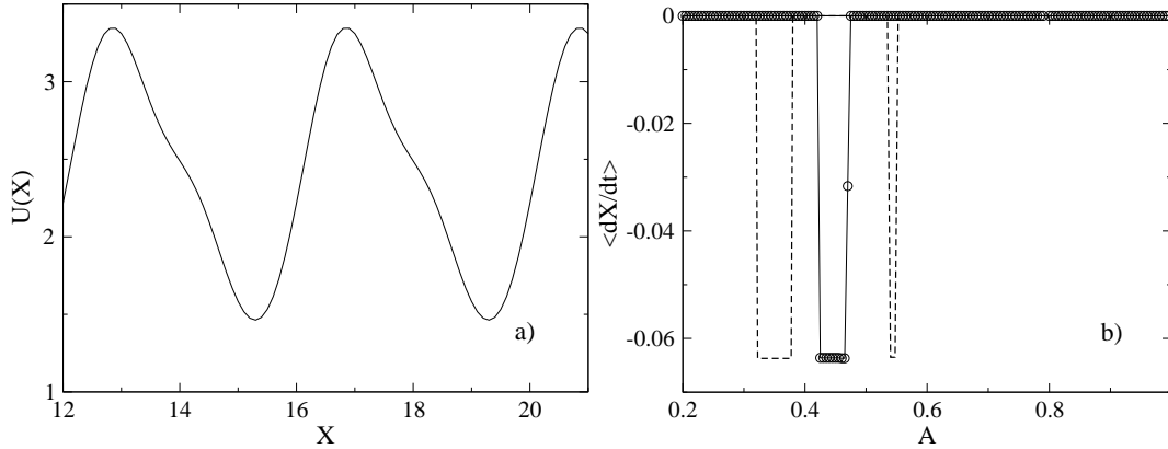
Fig. 1 – a) Effective potential for the kink center within the adiabatic approach, originating in the perturbation V(x) defined in Eq. (3) with \epsilon = 0.8 , x_1 = 0.5 , x_2 = 1. , x_3 = 2.3 and period L = 4 . b) Mean kink velocity \langle dX/dt \rangle vs driving amplitude A for the frequency \omega = 0.1 . Circles: direct numerical simulation of Eq. (1), the line being only a guide to the eye; dashed line: collective coordinate approach, Eq. (4).
