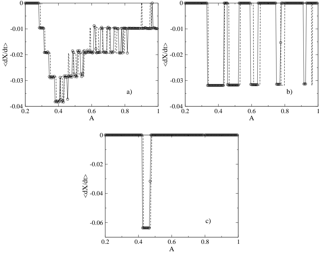
Fig. 2 – Mean kink velocity \langle dX/dt \rangle vs driving amplitude A for different frequencies: a) \omega = 0.015 , b) \omega = 0.05 , c) \omega = 0.1 . Other parameters are the same as in Fig. 1. Circles: direct numerical simulation of Eq. (1), the line being only a guide to the eye; dashed line: improved collective coordinate theory, Eqs. (11), (12).
