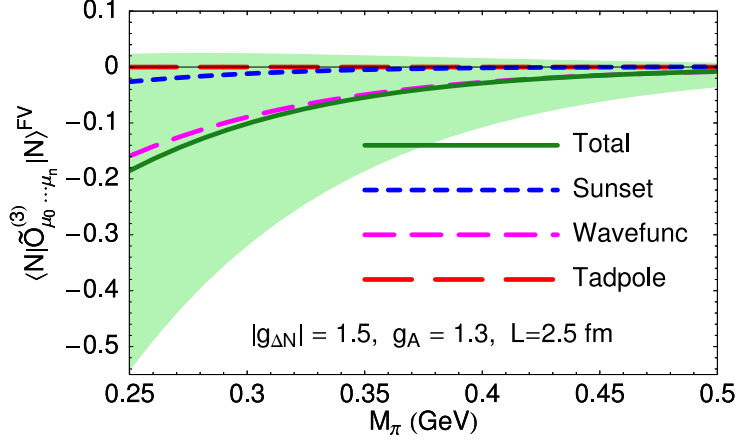
FIG. 7: Finite volume effects in the isovector, helicity matrix elements in the proton in SU(2|2) quenched \chi PT. The shaded region corresponds to variation of the axial couplings g_1 and \gamma between \pm g_A with g_A = 1.3 , g_{\Delta N} = 1.5 and assuming large N_c relations for the operator LECs. The point M_\pi = 0.25 GeV corresponds to M_\pi L = 3.2 .
