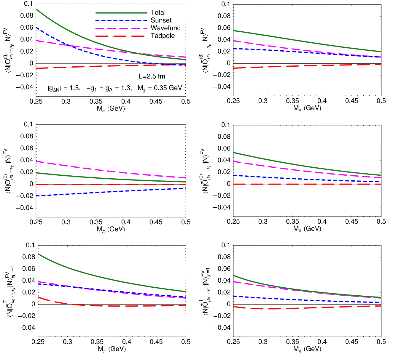
FIG. 5: As in Fig. 4 except with g_1 = -g_A . M_\pi = 0.25 GeV corresponds to M_\pi L = 3.2 .
