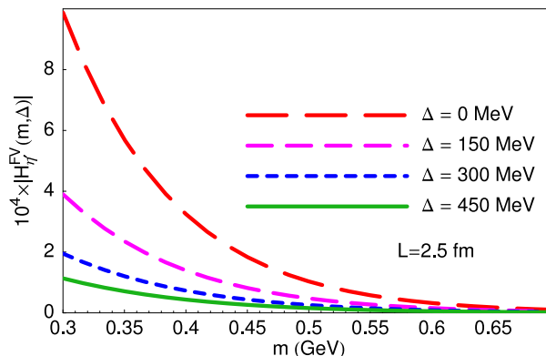
FIG. 3: Dependence of finite volume effects in double-pole contributions on the mass-splitting \Delta . Note that the scale here is ten times that in Fig. 2. The point m = 0.3 GeV corresponds to mL = 3.8 .
