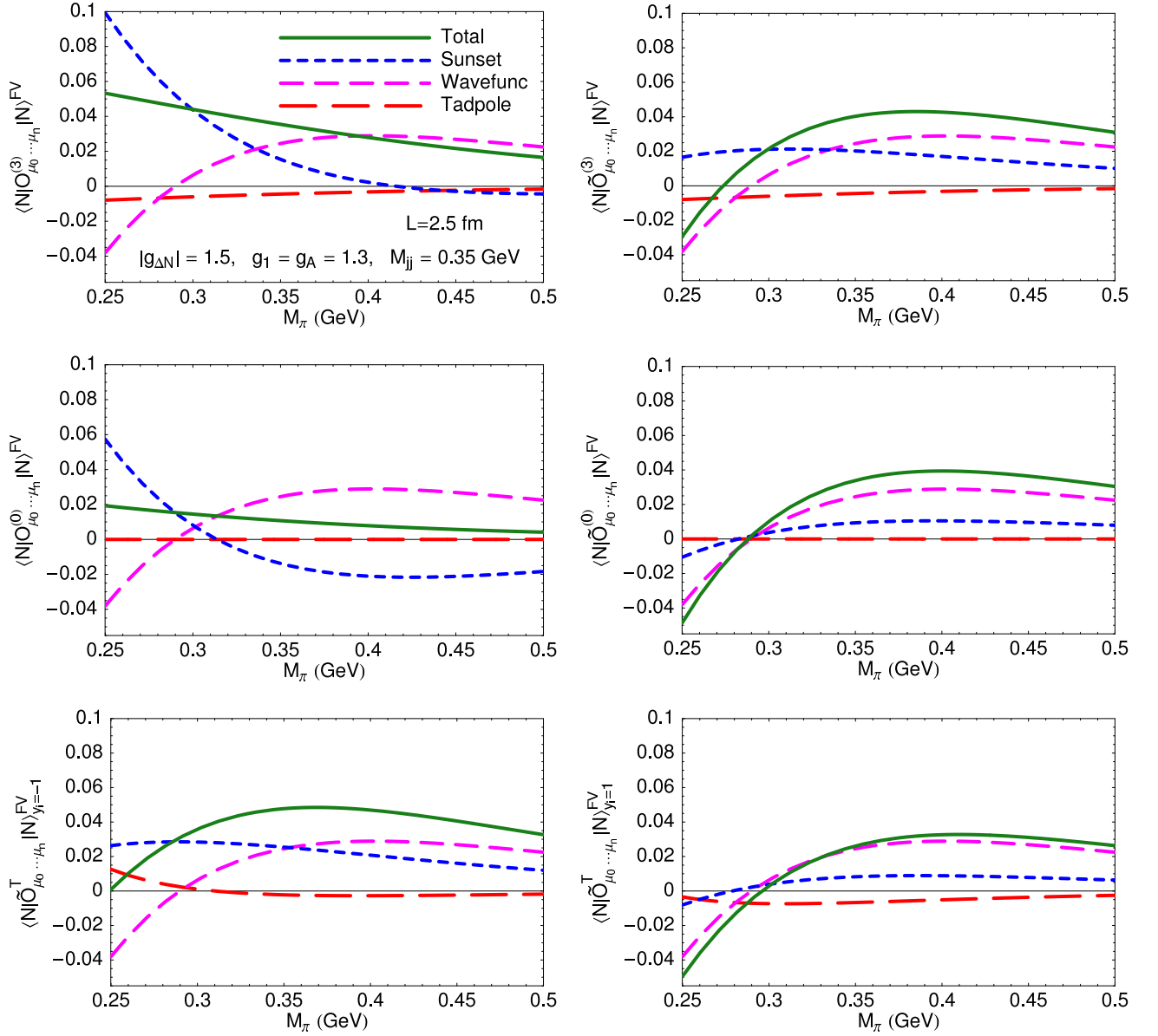
FIG. 4: Indicative finite volume effects in SU(4|2) matrix elements. The results in the first row are for the isovector unpolarised (left) and helicity (right) operators and those in the second row are similarly for the isoscalar unpolarised (left) and helicity (right) operators. The third row corresponds to the transversity “isovector” y_i = -1 (left) and “isoscalar” y_i = 1 (right) matrix elements. In each plot, the solid curve shows the total result, whilst the short-, medium- and long-dashed curves correspond to the individual FV effects arising from diagrams (c)–(f), diagrams (a) and (b), and diagram (i) in Fig. 1. In all of these results, we have considered a (2.5 \text{ fm})^3 box and set g_A = g_1 = 1.3 and |g_{\Delta N}| = 1.5 . M_\pi = 0.25 \text{ GeV} corresponds to M_\pi L = 3.2 .
