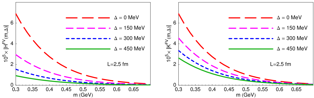
FIG. 2: Dependence of finite volume effects on the mass-splitting \Delta in individual integrals/sums corresponding to diagrams (a)—(f) in Fig. 1. The point m = 0.3 GeV corresponds to mL = 3.8 .
