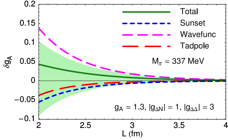
FIG. 6: Finite volume effects in QCD calculations of g_A at M_\pi = 337 MeV (as appropriate for the recent LHP simulations [59]). L = 2 fm corresponds to M_\pi L = 3.4 . The shaded region corresponds to varying 1.0 \leq g_A \leq 1.5 , 0 \leq |g_{\Delta N}| \leq 2 .
