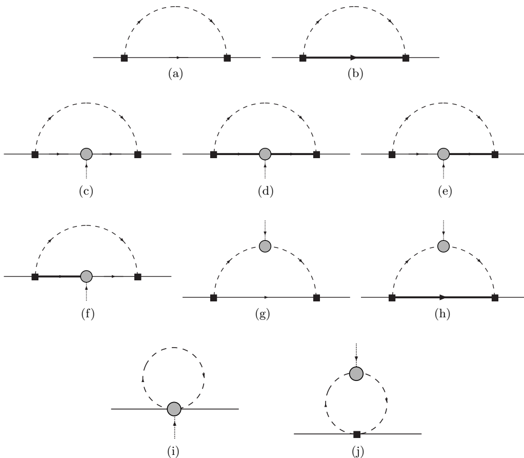
FIG. 1: Diagrams contributing to nucleon matrix elements of the twist-two operators. The black square corresponds to an interaction from the strong Lagrangian and the gray circle represents an insertion of the twist-two operators in Eqs. (18)–(20). The thin, thick and dashed lines are \mathbf{70} -plet baryons, \mathbf{44} -plet baryons and mesons respectively. The first two diagrams represent the wave-function renormalisation and the remainder are operator renormalisations. Diagrams (e) and (f) are absent for the unpolarised, and isoscalar operator matrix elements, and diagrams in which the twist-two operator is inserted on a meson line are only present in the unpolarised case.
