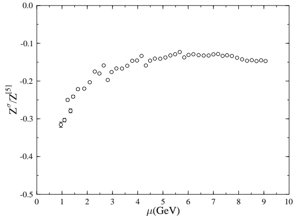
FIG. 3: The ratio Z^\sigma(a\mu)/Z^{\{5\}}(a\mu) at \beta = 5.40
