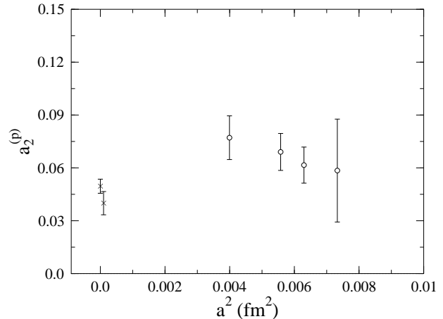
FIG. 4: The chirally extrapolated reduced matrix element a_2 for the proton target renormalized at the scale \mu^2 \equiv Q^2 = 5 \text{ GeV}^2 as a function of the lattice spacing a . The crosses denote phenomenological determinations.
