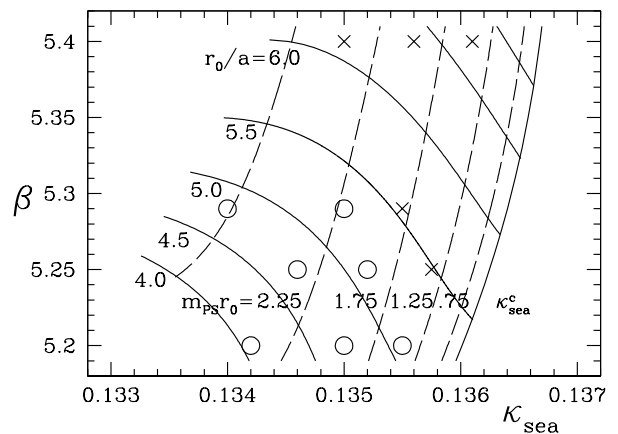
FIG. 1: Parameters of our dynamical gauge field configurations, together with lines of constant r_0/a (solid lines) and lines of constant m_{\text{PS}} r_0 (dashed lines). The simulations are done on 24^3 \times 48 ( \times ) and 16^3 \times 32 ( \circ ) lattices, respectively.
