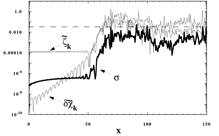
FIG. 3. Threshold PBH formation – the growth of \sigma , \tilde{\zeta}_k \equiv k^{3/2}\zeta_k , and \delta\tilde{\chi}_k \equiv k^{3/2}\delta\chi_k/m_{\text{pl}} for a super-Hubble mode \kappa \equiv k/(\sqrt{\lambda}\phi_0) = 10^{-22} vs dimensionless time x \equiv \sqrt{\lambda}\phi_0\eta in the case g^2/\lambda = 2.5 , where \phi_0 \simeq 0.1m_{\text{pl}} is the value of inflaton when it begins to oscillate coherently. With the choice k_* = aH in the window function \tilde{W}(kR) = \exp(-k^2 R^2/2) , \sigma just reaches the threshold \sigma_* = 0.03 for the PBH formation for chi-squared first order distributions.
