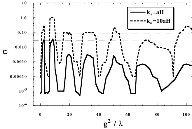
FIG. 5. The mass variance \sigma vs g^2/\lambda for two window function cut-offs k_* = aH and k_* = 10aH . The threshold of \sigma_* = 0.03 in the chi-squared distributed case is shown and is marginally crossed for the regions around g^2/\lambda \sim 2 and g^2/\lambda \sim 8 when k_* = aH . For k_* = 10aH a quilt of regions above the Gaussian threshold \sigma_* = 0.08 emerges which coincide closely with g^2/\lambda = 2n^2 corresponding to Floquet indices with maxima at longest wavelengths.
