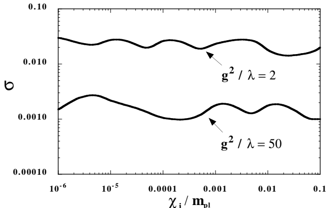
FIG. 6. The smoothed dependence of the final mass variance \sigma on the initial condition, \chi_i , 55 e-folds before the start of preheating for g^2/\lambda = 2, 50 . Note the relatively weak dependence in both cases.
