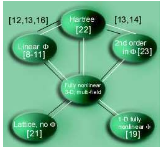
FIG. 1. A schematic figure showing the numerical approaches to preheating with numbers in brackets denoting appropriate references. See the text for discussion.
