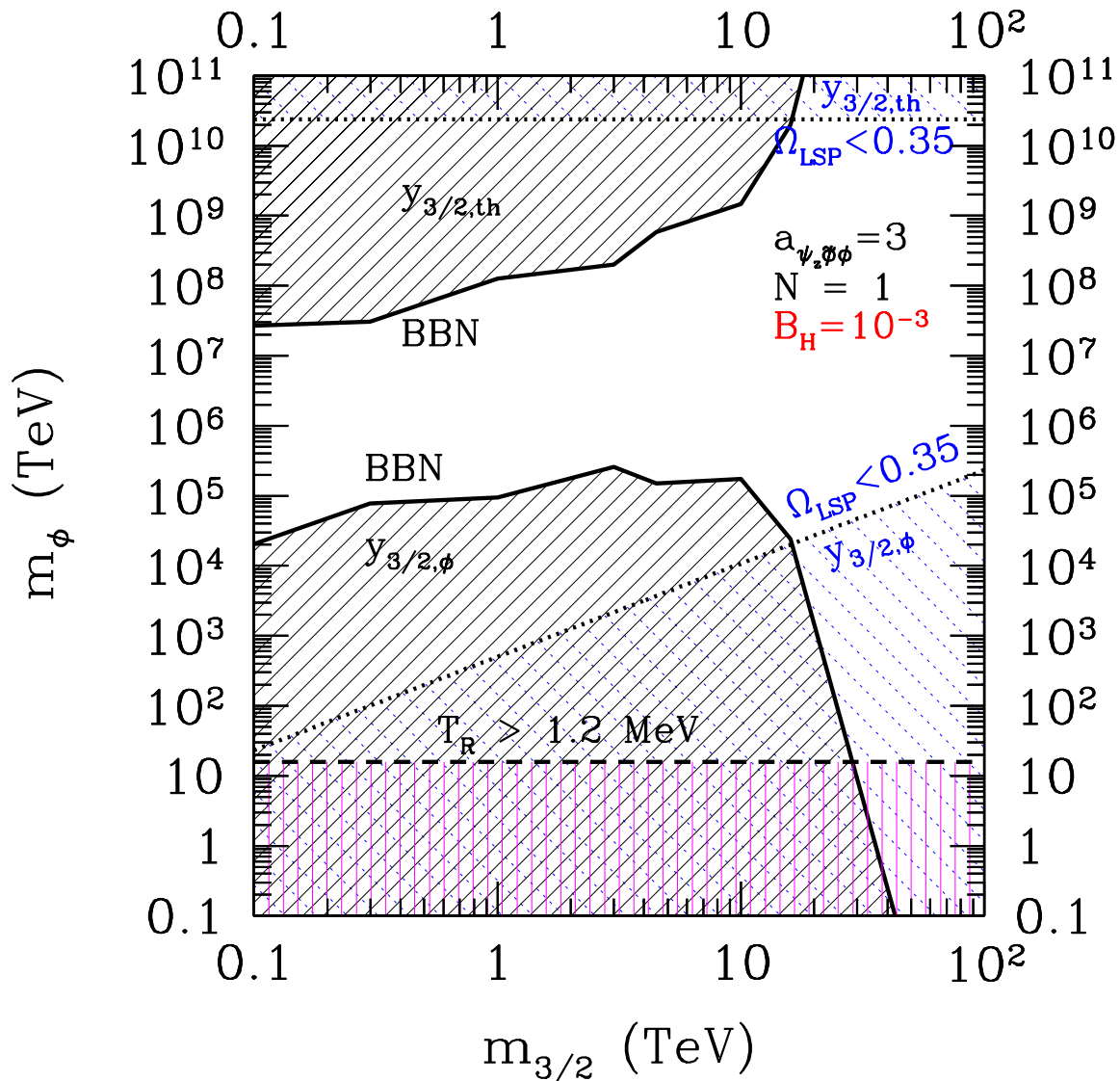
FIG. 1. Constraints on modulus mass m_\phi as a function of gravitino mass m_{3/2} in case that the hadronic branching ratio is B_H = 10^{-3} . The solid lines denote the limits which come from the photodissociation and hadro-dissociation effects on light elements by the decaying gravitino (BBN). The dotted lines represent constraints on the energy density for LSPs, which are produced by decaying gravitinos, to satisfy \Omega_{\text{LSP}} < 0.35 for m_{\text{LSP}} = 100 GeV. The dashed line denotes the lower bound on m_\phi arising from the lower bound on the reheating temperature after modulus decay to thermalize the neutrino background for successful BBN ( T_R > 1.2 MeV). Here we adopted a_{\psi_z \tilde{\phi} \phi} = 3 and N = 1 . We also assumed that the abundance of the gravitinos produced through the reheating process after the primordial inflation are negligible. This corresponds to the case that the reheating temperature after primordial inflation is sufficiently low, T_R^{\text{inf}} = 0 - 10^{12} GeV, or J < J_{\text{cr}} .
