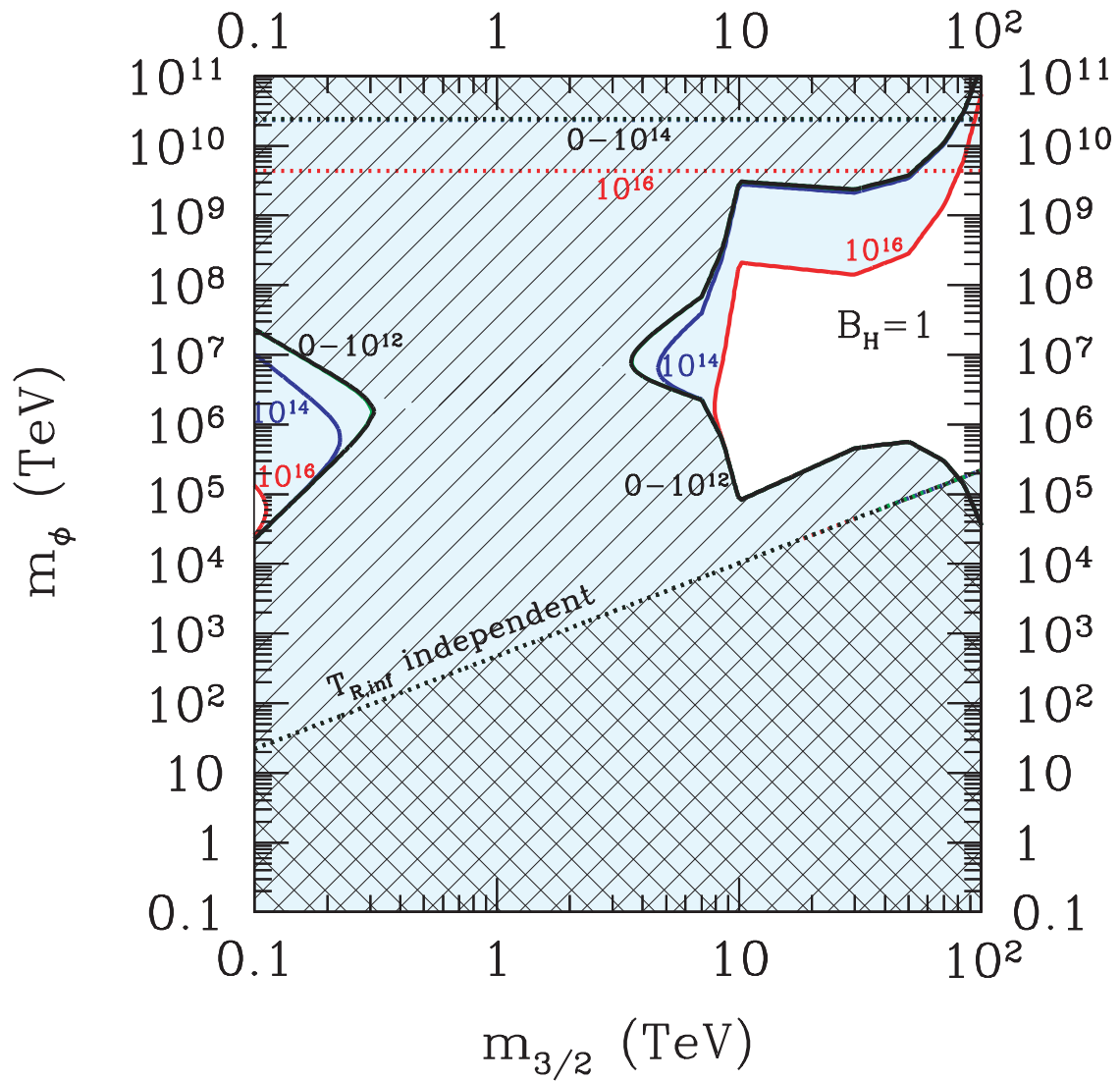
FIG. 4. Same as Fig. 2, but for B_H = 1
