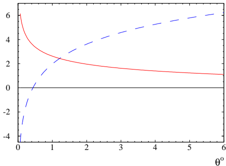
FIG. 1: Logarithmically enhanced (dashed line) and nonlogarithmic (solid line) second order corrections to the differential cross section of the small angle Bhabha scattering as functions of the scattering angle for \sqrt{s} = 100 GeV and \ln(\varepsilon_{cut}/\varepsilon) = 0 , in units of 10^{-3} .
