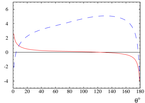
FIG. 2: The same as Fig. (1) but for the large angle Bhabha scattering and \sqrt{s} = 1 GeV.
