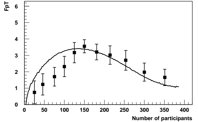
Fig. 3. F_{pt}(0/0) vs the number of participants. Experimental data from PHENIX at \sqrt{s} = 200 GeV . Solid line our results.
