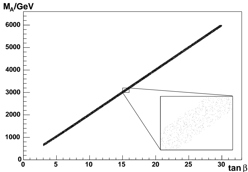
Figure 1: The distribution of scenarios with physically acceptable vacua, with M_A chosen randomly between 0 and 6 TeV, \tan \beta chosen randomly between 3 and 30 and \mu = 200 GeV. The blow-up allows individual scenario points to be seen.
