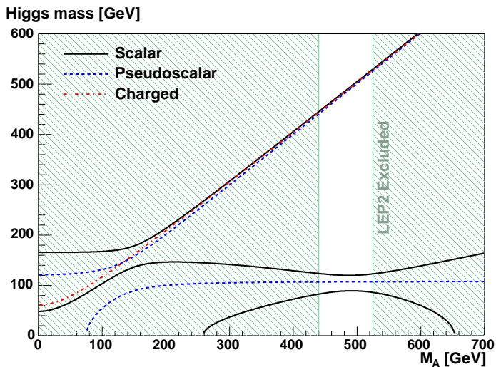
Figure 2: The dependence of the Higgs boson masses on m_A for \lambda = 0.3 , \kappa = 0.1 , \mu = 157 GeV, \tan \beta = 3 and A_\kappa = -60 GeV. Solid, dashed and dashed-dotted curves correspond to the one-loop masses of the CP-even, CP-odd and charged Higgs bosons respectively. All masses are given in GeV.
