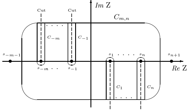
Figure 1: System of contours on the complex- z plane.
