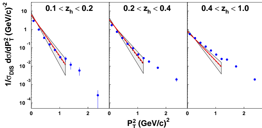
FIG. 5: The normalized cross section d\sigma/dP_T^2 : the dashed line is obtained with exact kinematics, while the solid bold line includes terms up to \mathcal{O}(k_\perp/Q) only. The shadowed region corresponds to varying the parameters \langle k_\perp^2 \rangle and \langle p_\perp^2 \rangle , given in Eq. (47) of the text, by 20%. The data are from Ref. [31].
