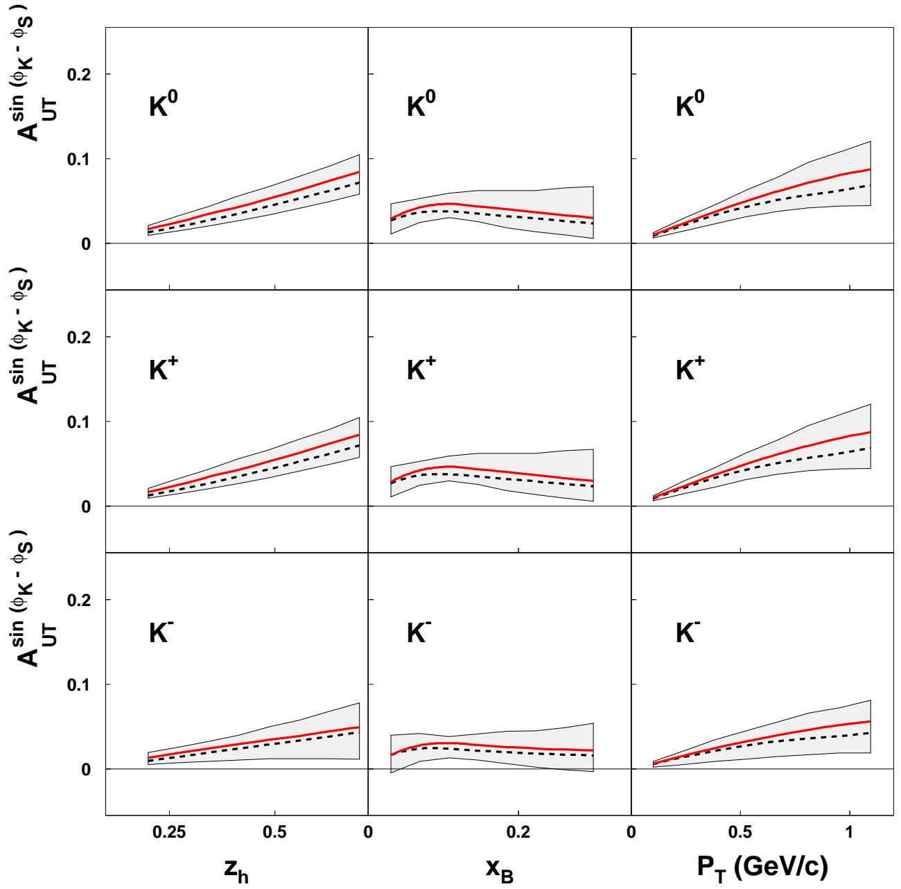
FIG. 9: Predictions for kaon asymmetries A_{UT}^{\sin(\phi_h - \phi_S)} at HERMES kinematics for scattering off a transversely polarized proton target. The curves correspond to calculation with exact kinematics (dashed line) or keeping only terms up to \mathcal{O}(k_\perp/Q) (solid bold line). The shadowed region corresponds to the theoretical uncertainty due to the parameter errors.
