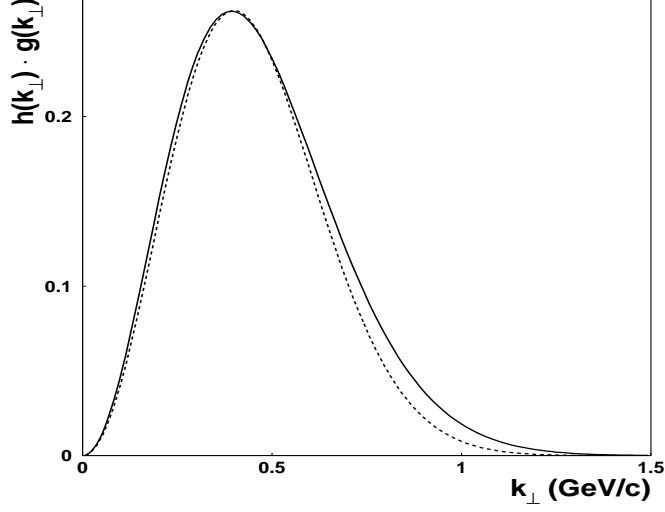
FIG. 7: The product h(k_\perp) \cdot g(k_\perp) , solid line, compared with the product h'(k_\perp) \cdot g(k_\perp) , dashed line, as a function of k_\perp .
