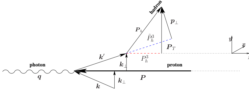
FIG. 2: Kinematics of the fragmentation process.
