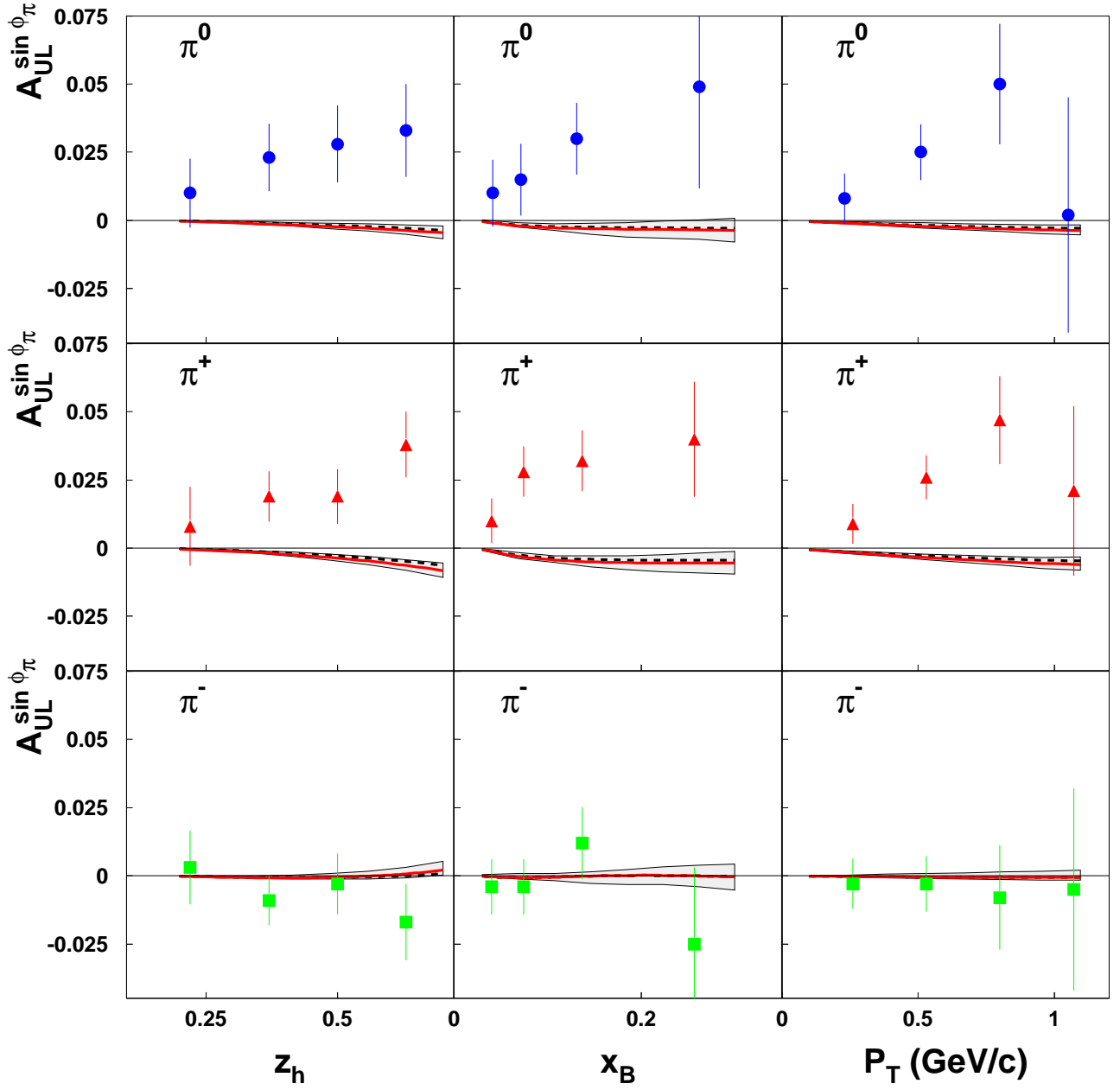
FIG. 11: HERMES data on A_{UL}^{\sin \phi_\pi} [9] for scattering off a longitudinally polarized proton target and pion production. The curves show the contribution of our Sivers functions alone, with exact kinematics (Eq. (57), dashed line) or keeping only terms up to \mathcal{O}(k_\perp/Q) (solid bold line). The shadowed region corresponds to the theoretical uncertainty due to the parameter errors.
