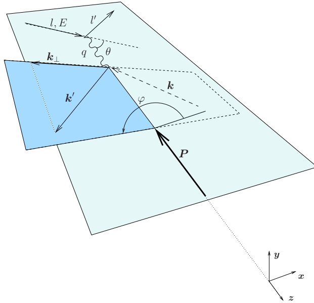
FIG. 1: Kinematics of DIS processes.
