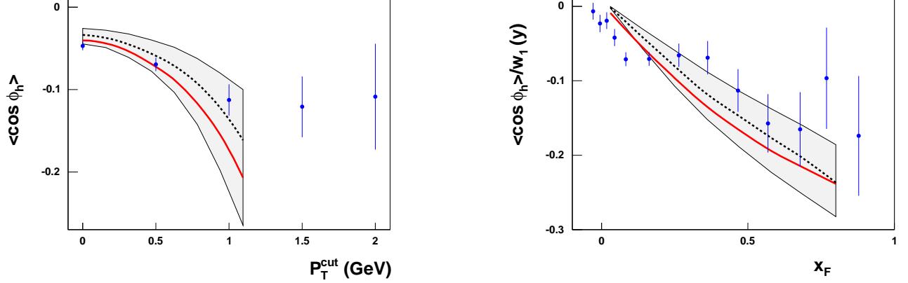
FIG. 6: \langle \cos \phi_h \rangle , as given by Eq. (44), as a function of P_T^{\text{cut}} , left panel, and x_F , right panel: the dashed line is obtained with exact kinematics, while the solid bold line includes terms up to \mathcal{O}(k_\perp/Q) only. The shadowed region corresponds to varying the parameters \langle k_\perp^2 \rangle and \langle p_\perp^2 \rangle , given in Eq. (47) of the text, by 20%. w_1(y) = \frac{(2-y)\sqrt{1-y}}{1+(1-y)^2} . The data are from Ref. [24], left panel, and Ref. [6], right panel.
