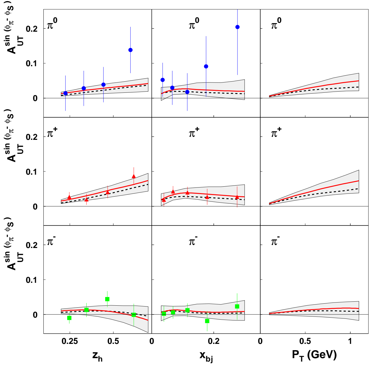
FIG. 8: HERMES data on A_{UT}^{\sin(\phi_\pi - \phi_S)} [10] for scattering off a transversely polarized proton target and pion production. The curves are the results of our fits, with exact kinematics (dashed line) or keeping only terms up to \mathcal{O}(k_\perp/Q) (solid bold line). The shadowed region corresponds to the theoretical uncertainty due to the parameter errors. Data on the P_T dependence of A_{UT}^{\sin(\phi_\pi - \phi_S)} are not available yet, and the third column of the figure gives our predictions.
