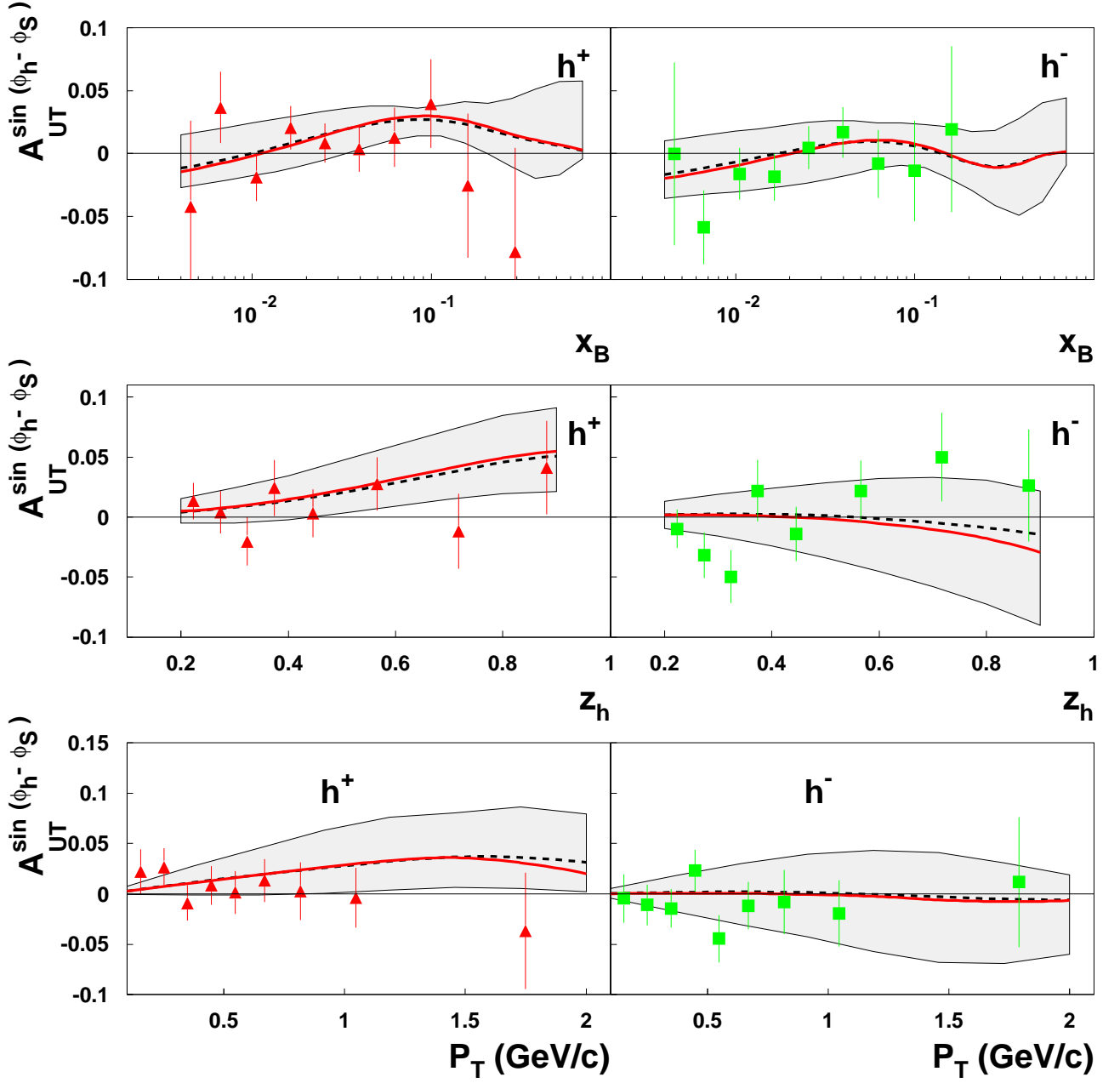
FIG. 10: COMPASS preliminary data [16] on A_{UT}^{\sin(\phi_h - \phi_S)} for scattering off a transversely polarized deuteron target and the production of positively ( h^+ ) and negatively ( h^- ) charged hadrons. The curves show our predictions, according to the values of the parameters for the Sivers functions given in Table 1 and obtained from fitting the HERMES data on A_{UT}^{\sin(\phi_\pi - \phi_S)} . Again, the dashed line refers to exact kinematics, Eq. (58), while the solid bold line is obtained by keeping only terms up to \mathcal{O}(k_\perp/Q) . The shadowed region shows the theoretical uncertainty due to the parameter errors.
