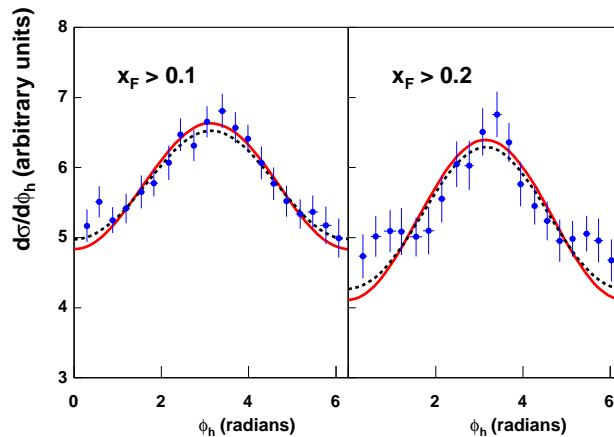
FIG. 4: Fits to the \cos \phi_h dependence of the cross section: the dashed line is obtained with exact kinematics, while the solid bold line includes terms up to \mathcal{O}(k_\perp/Q) only. The data are from Ref. [6].
