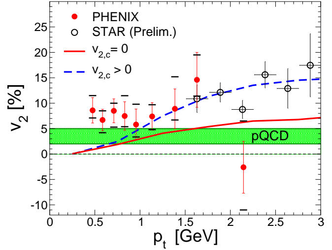
Fig. 2. Azimuthal asymmetry of “non-photonic” single- e^\pm spectra in minimum bias Au - Au ( \sqrt{s_{NN}} = 200 GeV) [28, 29] compared to coalescence model predictions [25] using c -quark distributions from either p - p collisions ( v_2^c = 0 , solid line) or assuming a transverse flow and v_2 -profile as determined for light quarks from fits to light-hadron spectra ( v_2^c > 0 , dashed line). The band indicates predictions from jet-quenching [24] applicable at sufficiently high p_t .
