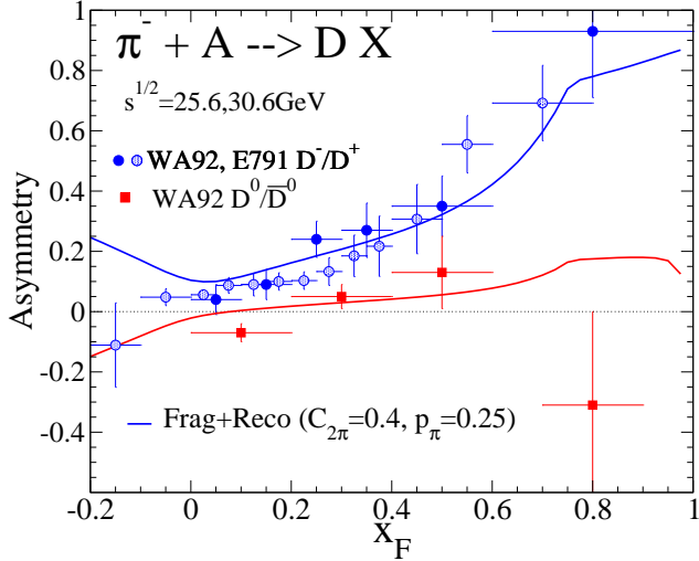
Fig. 1. D -meson flavor asymmetries, A = (N_{D_1} - N_{D_2}) / (N_{D_1} + N_{D_2}) , in \pi^- - A reactions [22,23] compared to coalescence + fragmentation calculations [6]. Upper data points and curves are for D_1 = D^- and D_2 = D^+ , whereas lower data points and curves are for D_1 = D^0 and D_2 = \bar{D}^0 . “Leading” particles ( D^- = \bar{c}d , D^0 = c\bar{u} ) are defined as sharing a valence quark with the projectile ( \pi^- = d\bar{u} ); note that the approximate absence of an asymmetry for D^0/\bar{D}^0 is accounted for in the model due to the predominant production of c\bar{c} pairs in the forward direction via \bar{u}u annihilation, rendering the valence \bar{u} unavailable for recombination.
