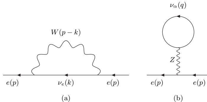
FIG. 3: One-loop diagrams for the electron self-energy in a neutrino gas.
