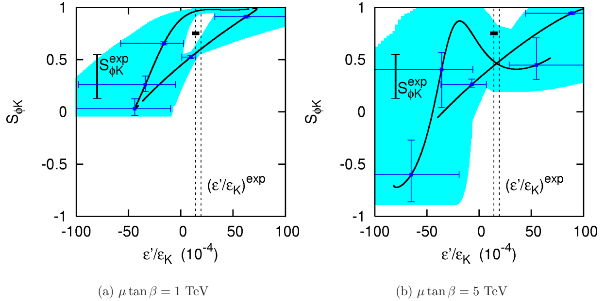
FIG. 2: S_{\phi K} vs. \text{Re}(\epsilon'/\epsilon_K) for (a) \mu \tan \beta = 1 \text{ TeV} and (b) \mu \tan \beta = 5 \text{ TeV} , with \tilde{m} = m_{\tilde{g}} = 500 \text{ GeV} . Experimental bounds on \text{Re}(\epsilon'/\epsilon_K) and S_{\phi K} are depicted by the vertical dashed lines and the thick vertical error bar, respectively. Their SM predictions are marked by the black box, whose extent indicates their uncertainties. The black curve does not include hadronic uncertainties, and the gray region includes them. The respective uncertainties in \text{Re}(\epsilon'/\epsilon_K) and S_{\phi K} are shown by the horizontal and vertical error bars at some selected points.
