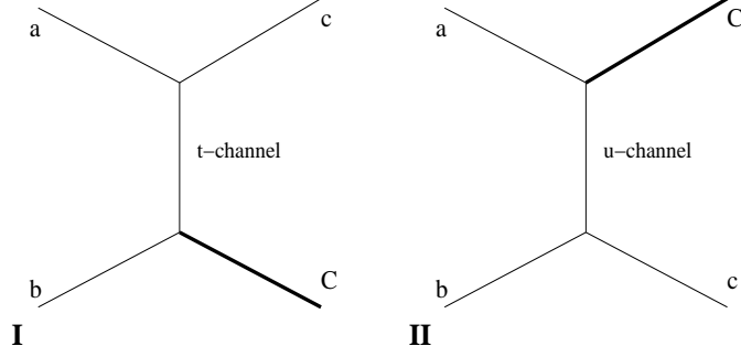
Figure 1: t - and u -channels for the process: a+b \rightarrow c+C (missing, closed-string state).
