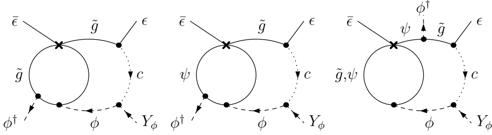
Figure 3: A two-loop diagram corresponding to ([S(\Gamma_{cl})] \cdot \Gamma^{\text{DRED}})_{\phi^\dagger \psi \bar{\epsilon}} . Such two-loop diagrams involving a virtual vector boson are the only ones where the \gamma -string B can contain three \gamma -matrices after integration over the fermion loop momentum.
