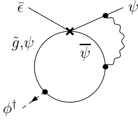
Figure 3: A two-loop diagram corresponding to ([S(\Gamma_{cl})] \cdot \Gamma^{\text{DRED}})_{\phi^\dagger \psi \bar{\epsilon}} . Such two-loop diagrams involving a virtual vector boson are the only ones where the \gamma -string B can contain three \gamma -matrices after integration over the fermion loop momentum.
