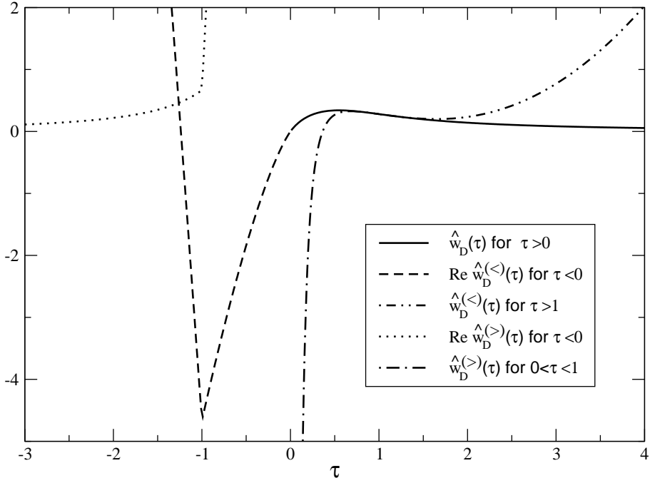
FIG. 1: The function \hat{w}_D(\tau) defined by (18) in the large \beta_0 approximation (i.e., with \hat{w}_D^{(<)}(\tau) and \hat{w}_D^{(>)}(\tau) given by (19)) is represented by a solid line. We separately display also the function \hat{w}_D^{(<)}(\tau) for \tau > 1 (dash-dot-dotted line) and for \tau < 0 (dashed line), and the function \hat{w}_D^{(>)}(\tau) for \tau < 1 (dash-dotted line and dotted line). For negative values of \tau the curves represent the real parts of the corresponding functions. The dashed line is unbounded for \tau tending to -\infty , while the dash-dot-dotted line grows unboundedly for \tau increasing. The dotted and dash-dotted lines are unbounded for \tau approaching zero from either side.
