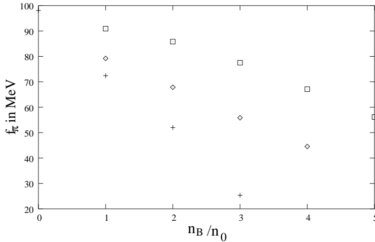
Figure 1: Density f_\pi from different models upto ( \sim 4\rho ) : diamonds corresponds to QCDSR results, + corresponds to the nuclear matter model of ZM, squares correspond to the SQM.
