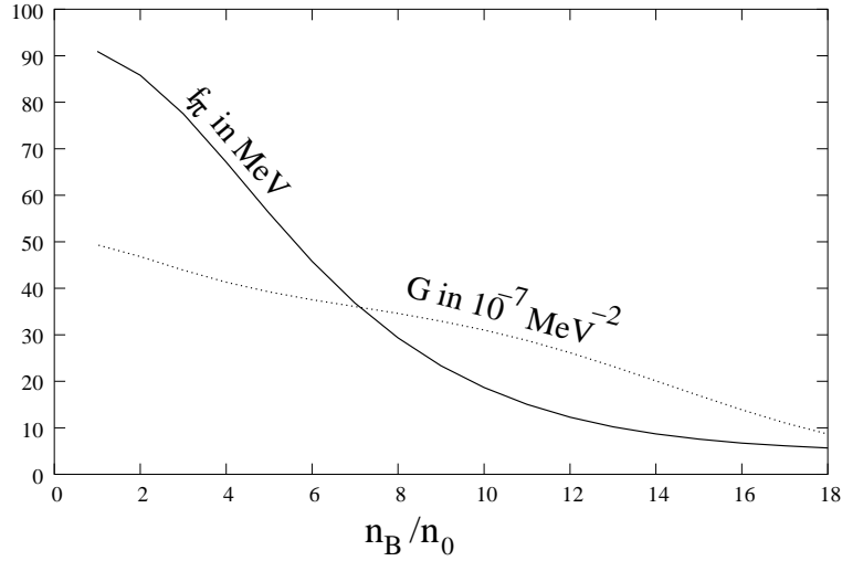
Figure 2: Predictions from density dependent quark mass of the SQM upto high density : density ( \rho ) dependence of f_\pi (full line), \rho dependence of the NJL coupling constant G (dotted line).
