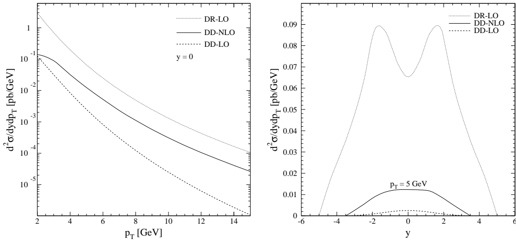
FIGURE 1. LO single-resolved (dotted lines), LO direct (dashed lines), and NLO direct (solid lines) contributions to d^2\sigma/dp_T dy (a) for y = 0 as a function of p_T and (b) for p_T = 5 GeV as a function of y .
