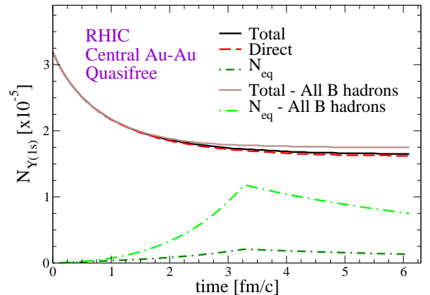
FIG. 19: (Color online) Same as Fig. 18 but assuming a richer (hadronic) open-bottom spectrum in the QGP as estimated from known open-charm hadrons in the vacuum.
