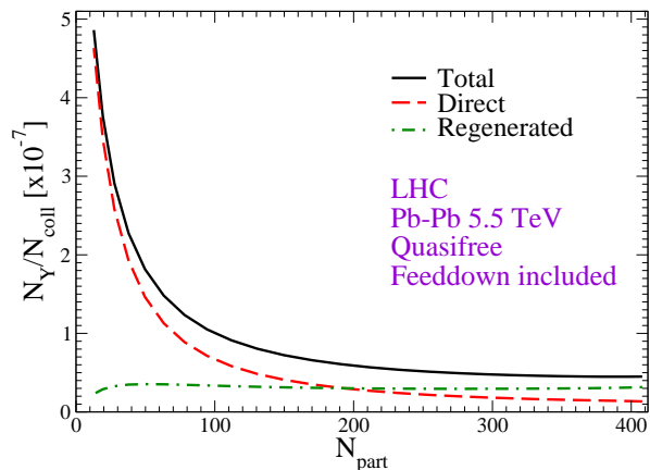
FIG. 15: (Color online) Same as Fig. 14, but for Pb-Pb collisions at LHC ( \sqrt{s_{NN}} = 5.5 TeV) with dN_{\text{ch}}/dy|_{\text{central}} \simeq 3200 .
