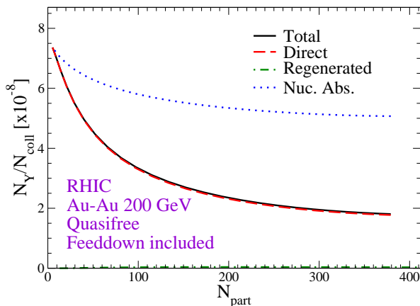
FIG. 14: (Color online) Centrality dependence of N_Y/N_{\text{coll}} at RHIC (Au-Au collisions at \sqrt{s_{NN}} = 200 GeV) using the quasifree suppression mechanism including color-screening. Dashed line: suppressed primordial \Upsilon . Dash-dotted line: regenerated \Upsilon . Solid line: total \Upsilon .
