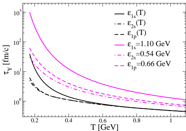
FIG. 5: (Color online) Y lifetimes computed from quasifree dissociation using constant (light set of curves) and in-medium (dark set of curves) binding energies for the Y (solid line), Y' (dash-dotted line) and the \chi_b (dashed line).
