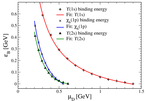
FIG. 3: (Color online) The dependence of Y binding energies (symbols) on gluon screening (Debye) mass according to solutions of the Schrödinger equation with a screened Cornell potential [33]. The lines indicate fits used for the numerical implementation in our calculations. The identification with temperature is provided by the perturbative expression for the Debye mass (see text), amounting to, e.g. , \mu_D(T_c) \simeq 325 MeV.
