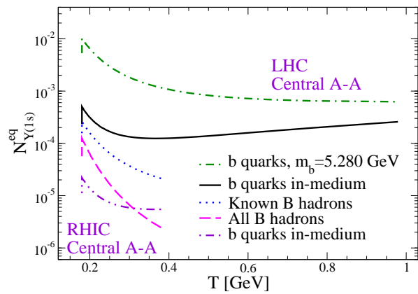
FIG. 7: (Color online) \Upsilon(1s) -equilibrium abundances for central A - A collisions at RHIC (lower 3 curves) and LHC (upper 2 curves), according to different scenarios for open-bottom states in the QGP (see text and App. C 1).
