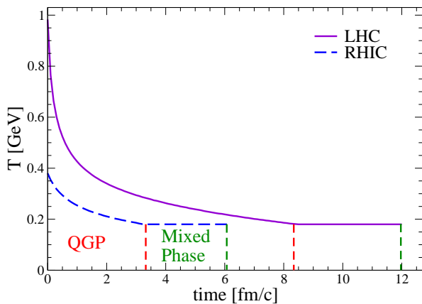
FIG. 6: (Color online) Time evolution of temperature within our expanding fireball model for a massive parton gas in central A - A collisions at RHIC (dashed line) and LHC (solid line). The use of massless partons (with N_f = 2.5 ) affects the evolution rather moderately.
