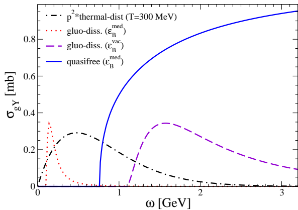
FIG. 1: (Color online) Gluo-dissociation (with vacuum binding energy: dashed line, or with in-medium reduced binding energy: dotted line) and quasifree (solid line) cross section overlap with a thermal gluon distribution at T = 300 MeV (dash-dotted line).
