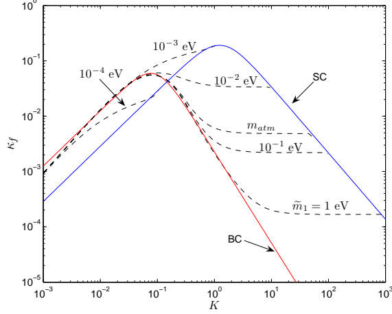
FIG. 2: (Color online) The efficiency factor K_f as a function of the decay parameter K , obtained by solving numerically the Boltzmann equations, for different values of the effective neutrino mass m_1 . The blue and red solid curves correspond to the numerical fits of K_f given in Eqs. (20), (21) and (22), for the cases of standard and brane cosmology, respectively.
