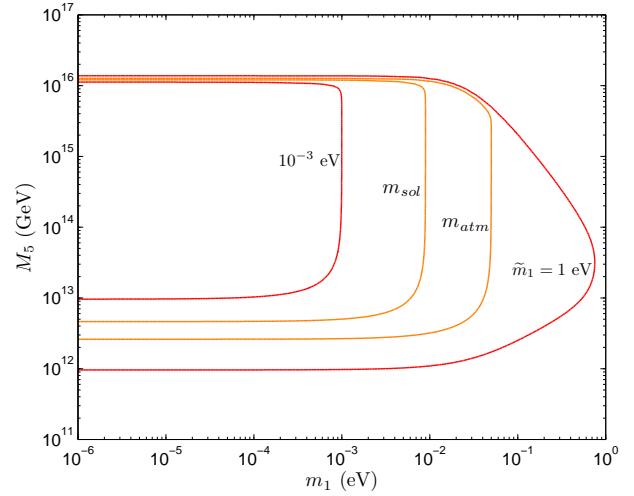
FIG. 3: (Color online) Contour lines of constant m_B^{\text{ax}} = m_B^{\text{obs}} = 5.8 \cdot 10^{10} in the (m_1; M_5) -plane for different values of \tilde{m}_1 . We assume that thermal leptogenesis occurs in the high-energy regime of brane cosmology.
