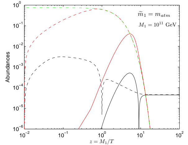
FIG. 1: (Color online) The evolution of N_{N_1} (red curves), N_{N_1}^{\text{eq}} (green curve) and j_{B=1j} (black curves) as functions of the temperature for M_1 = 10^{11} \text{ GeV} and m_1 = m_{\text{atm}} . The solid (dashed) lines correspond to the brane (standard) cosmology result.
