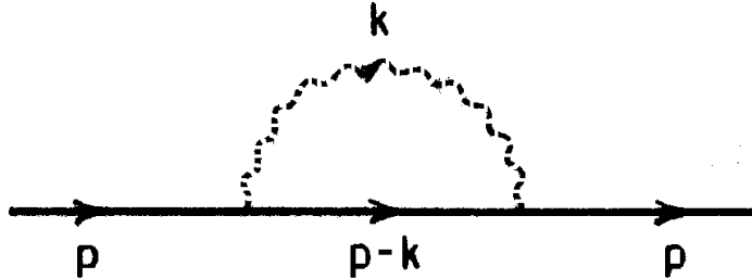
FIG. 2: The Feynman diagram for the contribution of a photonic tachyon to fermion self-energy. The wavy line denotes the tachyonic Kaluza-Klein modes of photon and the solid line denotes the fermion
