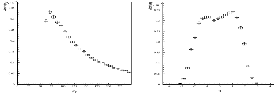
Fig. 6. Transverse momentum distribution (left panel) and rapidity distribution (right panel) of d -jet in u\bar{u} \rightarrow W^+W^-d\bar{d} process.
