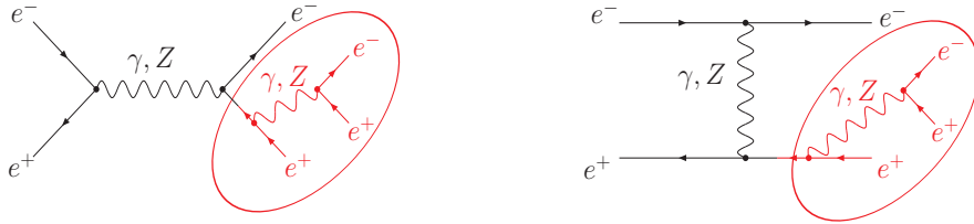
Fig. 1. An example of common parts of the amplitudes (in red) for the e^+e^- \rightarrow e^+e^-e^+e^- process.
