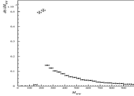
Fig. 5. Invariant mass distribution of the W^+W^- system in u\bar{u} \rightarrow W^+W^-d\bar{d} process.
