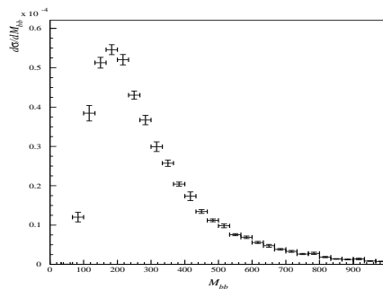
Fig. 3. Invariant mass distribution of the bb system in gg \rightarrow W^+W^-b\bar{b}b\bar{b} process.
