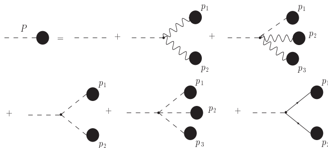
Fig. 2. Recursion equations for the Higgs boson.
