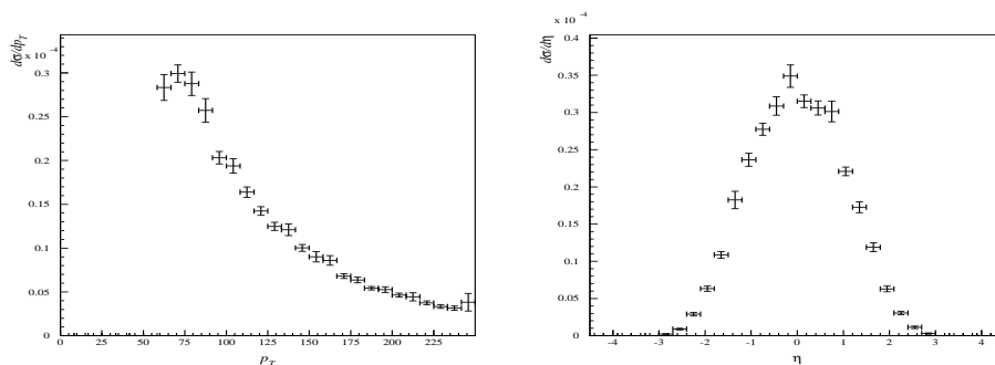
Fig. 4. Transverse momentum distribution (left panel) and rapidity distribution (right panel) of b -jet in gg \rightarrow W^+W^-b\bar{b}b\bar{b} process.
