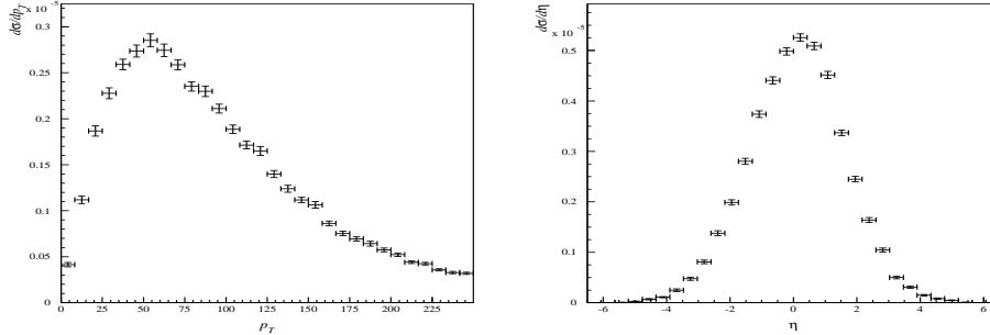
Fig.7. Transverse momentum distribution (left panel) and rapidity distribution (right panel) of W in u\bar{u} \rightarrow W^+W^-d\bar{d} process.
