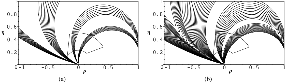
Figure 6: The solutions of the degree-four polynomial equation (72) in the (\rho, \eta) plane for the numerical example a_{\text{dir}} = 0.12 , \sin 2\alpha_{\text{eff}} = 0.58 and R_P = \lambda^2 \mathcal{B}_{K\pi^\pm} / \mathcal{B}_{\pi^+\pi^-} = 0.061 (see Appendix A). A guess value for the relative theoretical uncertainty on R_P in Eq. (109) is assumed: respectively 30% (a) and 60% (b), at the amplitude level. There are four families of curves corresponding to the two possible signs for \cos 2\alpha_{\text{eff}} , and to the cosine discrete ambiguity of Eq. (60) which is hidden in the polynomial (72). In the background is shown a crude representation of the early-1998 allowed domain [32].
