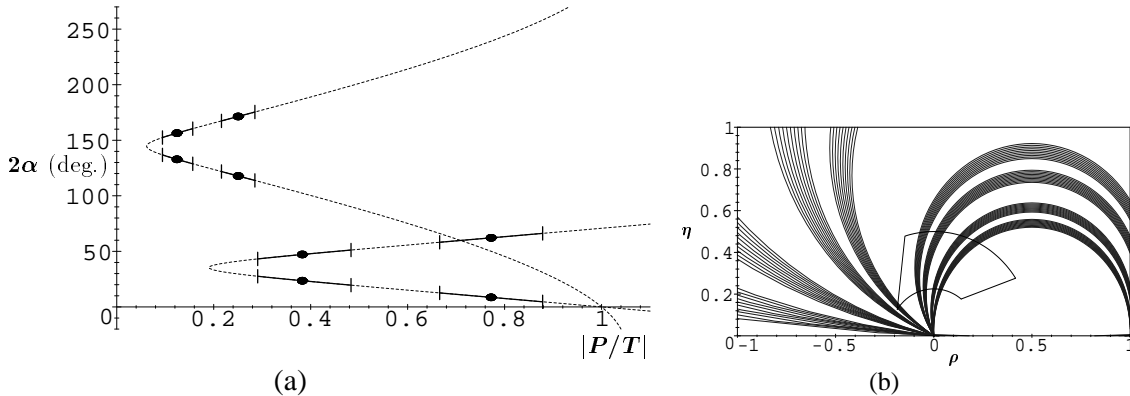
Figure 7: The eight solutions of the Gronau-London isospin analysis, for the numerical example a_{\text{dir}} = 0.12 , \sin 2\alpha_{\text{eff}} = 0.58 , \mathcal{B}_{\pi^{\pm}\pi^0}/\mathcal{B}_{\pi^+\pi^-} = 0.71 , \mathcal{B}_{\pi^0\pi^0}/\mathcal{B}_{\pi^+\pi^-} = 0.061 and a direct CP-asymmetry in the \pi^0\pi^0 channel equal to a_{\text{dir}}^{\pi^0\pi^0} = 0.32 (see Appendix A). (a) In the (|P/T|, 2\alpha) plane, the dots represent the central values obtained from Eqs. (112-114), while the solid curves (limited by the small dashes) represent the allowed domain when assuming that 2\alpha is affected by a 4^\circ uncertainty due to electroweak penguin contributions, as explained in the text. (b) The same allowed domain is represented in the (\rho, \eta) plane, where it is obtained by plotting the circle (98) for 2\alpha varying in the eight solution intervals. In the background is shown a crude representation of the early-1998 allowed domain [32].
