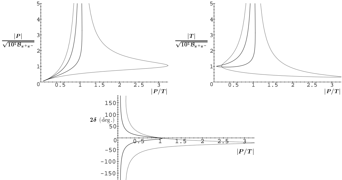
Figure 2: The |P| , |T| amplitudes and the strong phase 2\delta respectively as functions of |P/T| obtained from Eqs. (58) and (60-62), for the numerical example a_{\text{dir}} = 0.12 and \sin 2\alpha_{\text{eff}} = 0.58 (see Appendix A). The solid curves correspond to \cos 2\alpha_{\text{eff}} < 0 and the dashed ones to \cos 2\alpha_{\text{eff}} > 0 . Note that |P| and |T| diverge when 2\alpha \rightarrow 0 , |P/T| \rightarrow 1 because the CP-asymmetries a_{\text{dir}} and \sin 2\alpha_{\text{eff}} are kept fixed: |P| and |T| have to be very large to produce CP-violation with a small CP-phase \alpha .
