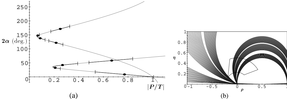
Figure 9: The eight solutions of the Buras-Fleischer analysis, for the numerical example a_{\text{dir}} = 0.12 , \sin 2\alpha_{\text{eff}} = 0.58 , a_{\text{dir}}^{K\bar{K}} = 0.21 , \sin 2\alpha_{\text{eff}}^{K\bar{K}} = 0.059 and \mathcal{B}_{K^0\bar{K}^0}/\mathcal{B}_{\pi^+\pi^-} = 0.058 (see Appendix A). (a) In the (|P/T|, 2\alpha) plane, the dots represent the central values obtained from Eqs. (123-124), while the solid curves (limited by the small dashes) represent the allowed domain when assuming that Eq. (121) is affected by a guess 30% relative uncertainty. Some of the solutions merge because of this theoretical error, leaving only six separate solutions. (b) The same allowed domain is represented in the (\rho, \eta) plane, where it is obtained by plotting the circle (98) for 2\alpha varying in the six solution intervals. In the background is shown a crude representation of the early-1998 allowed domain [32].
