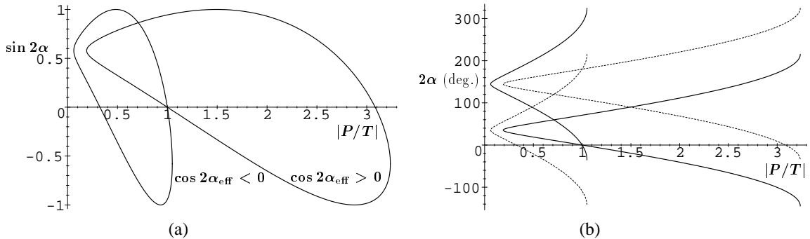
Figure 3: (a) \sin 2\alpha as a function of |P/T| obtained from Eq. (58), for the numerical example a_{\text{dir}} = 0.12 and \sin 2\alpha_{\text{eff}} = 0.58 (see Appendix A). The two branches corresponding to the two possible signs for \cos 2\alpha_{\text{eff}} are not degenerate. (b) 2\alpha as a function of |P/T| obtained by computing \arcsin(\sin 2\alpha) and \pi - \arcsin(\sin 2\alpha) : the comparison with Fig. 1 shows that the dashed curves are wrong solutions.
