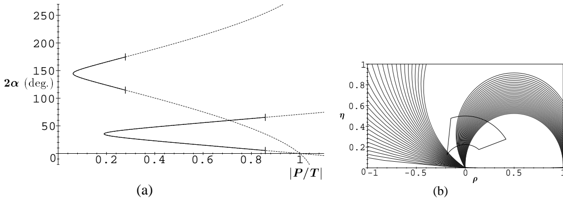
Figure 5: (a) The bound |2\alpha - 2\alpha_{\text{eff}}| \leq \Delta in the (|P/T|, 2\alpha) plane, obtained as explained in the text, for the numerical example a_{\text{dir}} = 0.12 , \sin 2\alpha_{\text{eff}} = 0.58 (see Appendix A) and \Delta = 30^\circ (solid curves limited by the small dashes). (b) The same bound in the (\rho, \eta) plane, obtained by plotting the circle (98) for 2\alpha varying in the interval [2\alpha_{\text{eff}} - \Delta, 2\alpha_{\text{eff}} + \Delta] . There are two families of circles corresponding to the two possible signs for \cos 2\alpha_{\text{eff}} . In the background is shown a crude representation of the early-1998 allowed domain [32].
