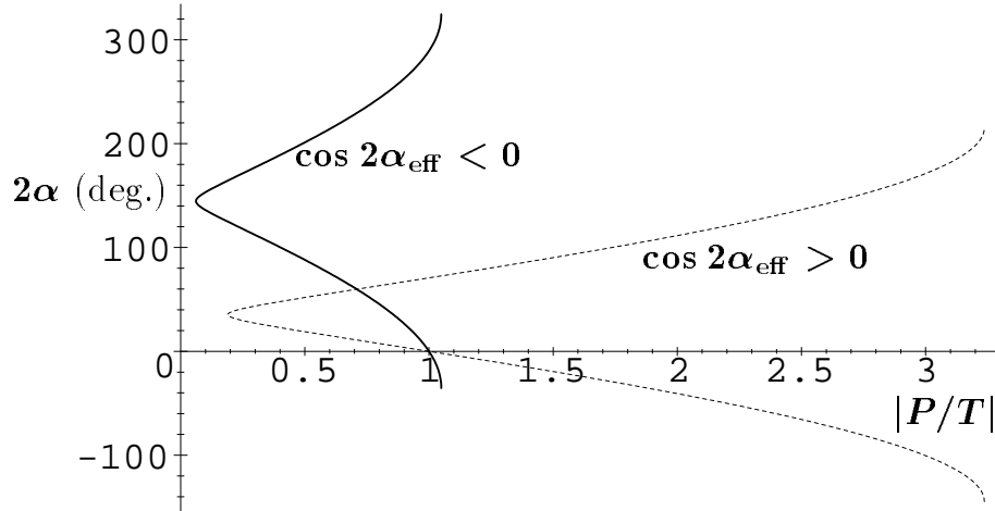
Figure 1: The CKM angle 2\alpha as a function of |P/T| obtained from Eq. (58), for a_{\text{dir}} = 0.12 and \sin 2\alpha_{\text{eff}} = 0.58 (see Appendix A for a description of this numerical example). The solid curve corresponds to \cos 2\alpha_{\text{eff}} < 0 and the dashed one to \cos 2\alpha_{\text{eff}} > 0 . Note that |P/T| varies in the range (63) which depends on the sign of \cos 2\alpha_{\text{eff}} . For a given value of |P/T| , there are in general four solutions for 2\alpha .
