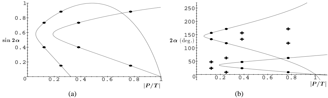
Figure 8: (a) The eight solutions of the isospin analysis in the (|P/T|, \sin 2\alpha) plane, for the same observables as in Fig. 7. (b) The solutions in the (|P/T|, 2\alpha) plane obtained by computing \arcsin(\sin 2\alpha) and \pi - \arcsin(\sin 2\alpha) : the comparison with Fig. 7 shows that the crosses are wrong solutions.
