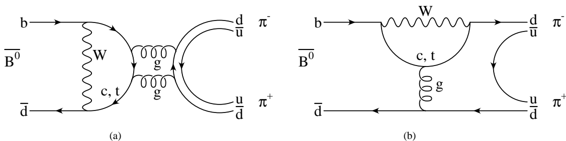
Figure 4: (a) OZI-suppressed annihilation penguin diagram. This diagram is OZI-suppressed and is neglected within Assumption 4 because it does not contribute to B \rightarrow K^\pm \pi^\mp . (b) Non-OZI-suppressed annihilation penguin diagram. This diagram is not OZI-suppressed, although it has annihilation topology. It is not neglected within Assumption 4 because it contributes to both B \rightarrow \pi^+ \pi^- and B \rightarrow K^\pm \pi^\mp .
