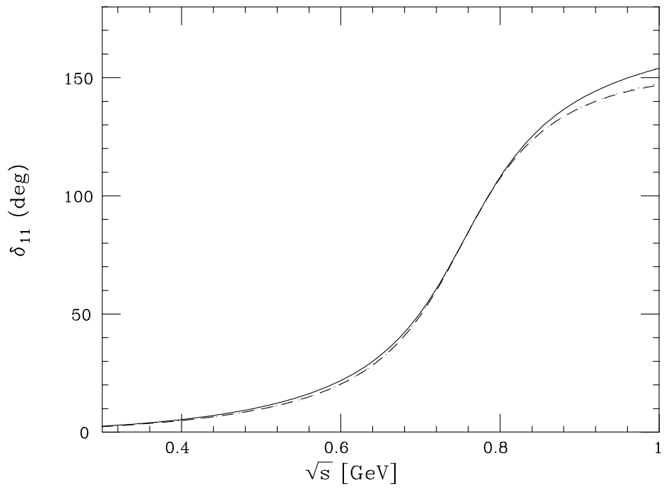
FIG. 1. The I = J = 1 \pi\pi phase shift. The solid curve is for only \rho exchange with the KSRF coupling, and the dashed (dotted) curve for degenerate \rho and \sigma with the Veneziano (KSRF/Weinberg) coupling. The latter two curves are almost indistinguishable.
