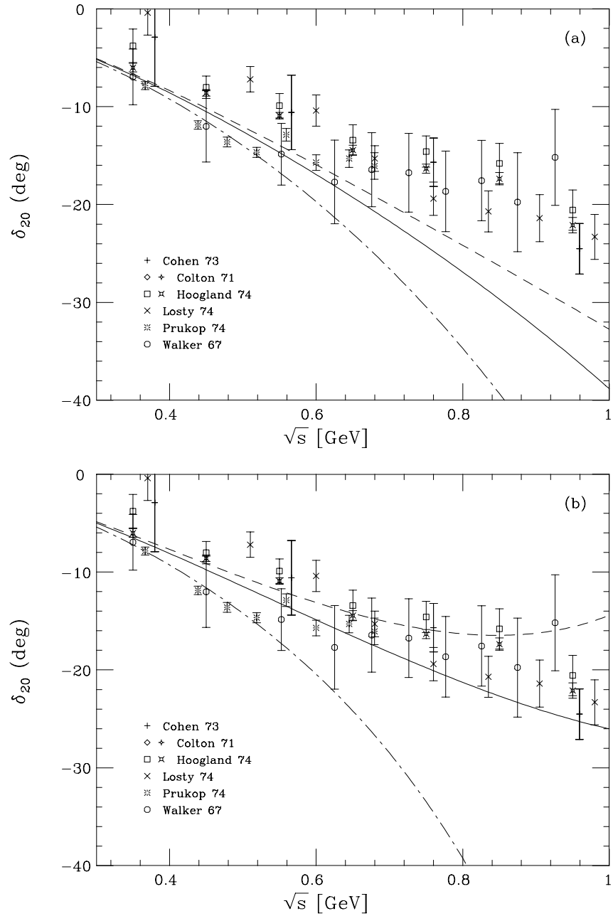
FIG. 3. The I=2, J=0 \pi\pi phase shift with (a) \rho exchange only; (b) degenerate \sigma and \rho exchanges for the KSUF/Weinberg (dashed), Veneziano (dot-dash), and intermediate g_\rho^2 = 0.45m_\rho^2/2f_\pi^2 (solid) couplings. Some experimental data are also shown.
