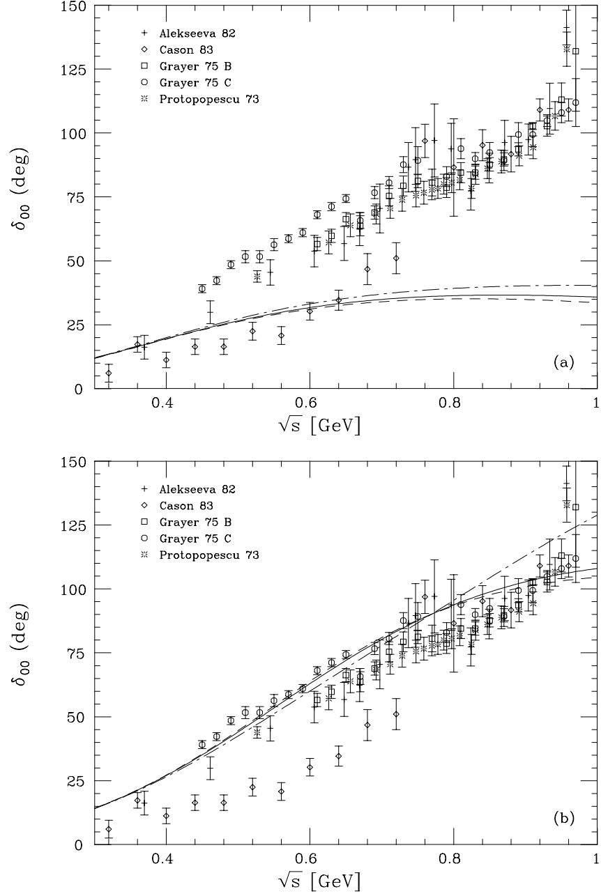
FIG. 2. The I = J = 0 \pi\pi phase shift with (a) \rho exchange only; (b) degenerate \sigma and \rho exchanges for the KSRF/Weinberg (dashed), Veneziano (dot-dash), and intermediate g_\rho^2 = 0.45m_\rho^2/2f_\pi^2 (solid) couplings. Some experimental data are also shown.
