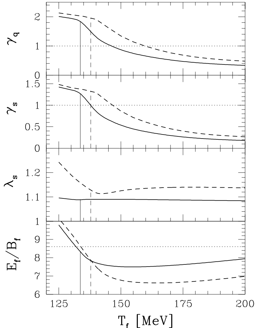
Figure 1: Variation of \gamma_q , \gamma_s , \lambda_s , and E_f/B_f , as function of temperature T_f , with all other parameters fixed by choosing best agreement with the experimental data.
