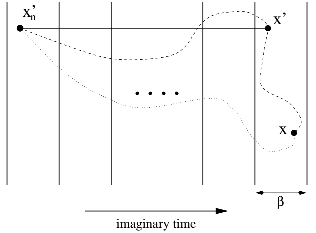
FIG. 1. The positions of the different points x , x' and x'_n are exhibited. The dotted line represents an arbitrary path from x'_n = x' - i\beta nu to x . As a first step, this path is continuously deformed in such a way that x' becomes an element of the path (dashed line). Secondly, the path from x'_n to x' can be deformed to a straight line (solid line), which gives rise to Eq. (19).
