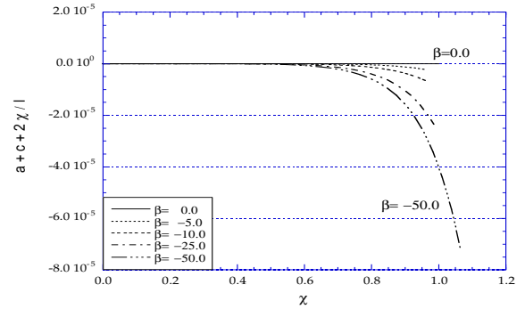
FIG. 3. The quantity a + c + 2\chi/l at r = r_+ plotted for M = 5 , Q = 0 and \beta = 0, -5, -10, -25 and -50 .
