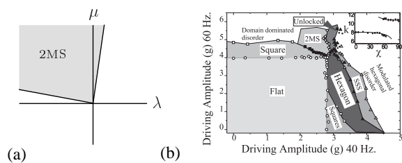
FIG. 5: (a) Region of stable 2MS under the assumptions of small damping, Hamiltonian structure, and supercriticality, (b) Experimental data, courtesy of J. Fineberg, reproduced from [6]. Since \lambda \sim |f_n| - |f_n|^{\text{crit}} and \mu \sim |f_m| - |f_m|^{\text{crit}} the orientation of the axes in (a) and (b) is the same.
