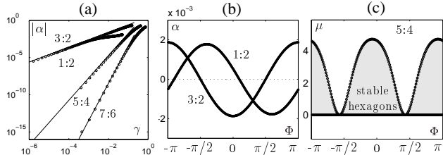
FIG. 3: Numerical calculations based on the Zhang Viñals equations (for a summary of the procedure see [10]). (a) |\alpha(\gamma)| for several choices of m:n [12]. Solid lines show predicted scalings. (b) \alpha(\Phi) for m:n = 1:2 and 3:2 , both with \gamma \simeq 0.001 . These cases have identical scaling in \gamma but are phase-shifted in \Phi . (c) Range of stable hexagons in Eqs. (6) for m:n = 5:4 and (realistic) parameters such that \gamma \simeq 0.245 .
