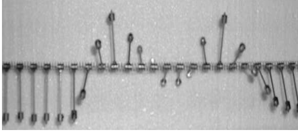
FIG. 5: Picture of a breather generated in a mechanical pendula chain driven at one end at a frequency in the forbidden band gap.
