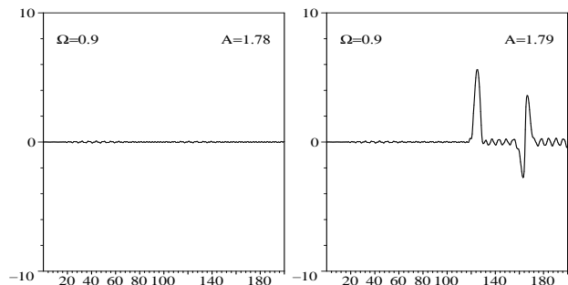
FIG. 2: Function u_n(t) for n = 60 in the case \Omega = 0.90 . The amplitude are A = 1.78 < A_s for the first figure and A = 1.79 = A_s for the second.
