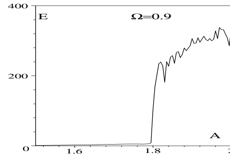
FIG. 1: Plot of the energy E injected in the sine-Gordon chain for T = 140 as a function of the driving amplitude A .
