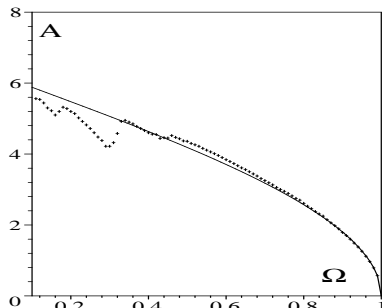
FIG. 3: Bifurcation diagram in the (A, \Omega) plane. The curve is the graph of formula (5). The points indicate the lowest amplitude for which nonlinear supratransmission starts.
