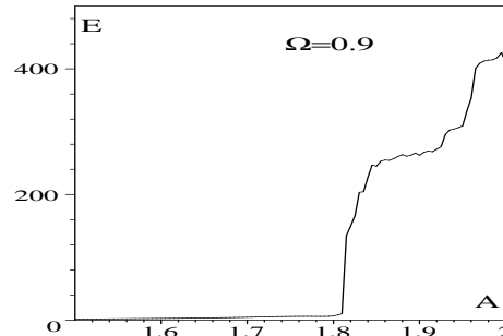
FIG. 4: Energy E injected in the Klein-Gordon nonlinear chain for T = 140 as a function of the driving amplitude A .
