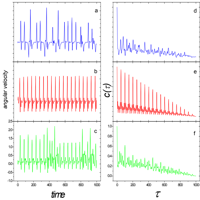
Fig. 2. Time series of the sixtieth pendulum (a, b, c) and the corresponding autocorrelation function time c(\tau) (d, e, f) with different disorder amplitude. (a), (d) \sigma = 0.0 ; (b), (e) \sigma = 0.3 ; (c), (f) \sigma = 0.6 .
