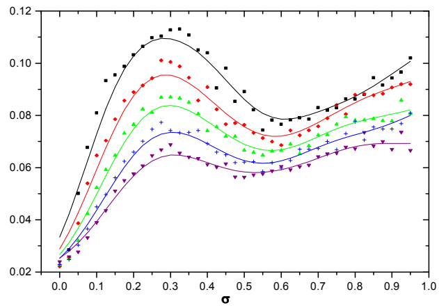
Fig. 4. The dependence of \tau(\sigma) on the disorder amplitude \sigma with noise intensity \beta of 0.1 (square), 0.3 (diamond), 0.5 (up triangle), 0.7 (cross), 0.9 (down triangle). Solid lines are drawn as a guide the eye.
