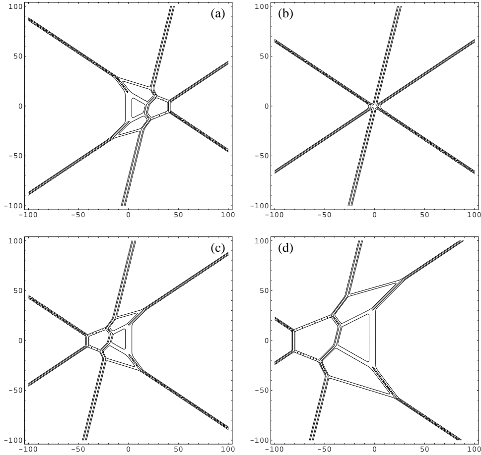
Figure 7. Snapshots illustrating the temporal evolution of a resonant 3-soliton solution u(x, y, t) with (k_1, \dots, k_6) = (-\frac{5}{2}, -\frac{3}{4}, -\frac{1}{2}, \frac{1}{2}, \frac{3}{2}, \frac{5}{2}) and \theta_1^0 = \dots = \theta_6^0 = 0 : (a) t = -10 , (b) t = 0 , (c) t = 10 , (d) t = 20 . Note the symmetry (x, y, t) \leftrightarrow (-x, -y, -t) in (a) and (c).
