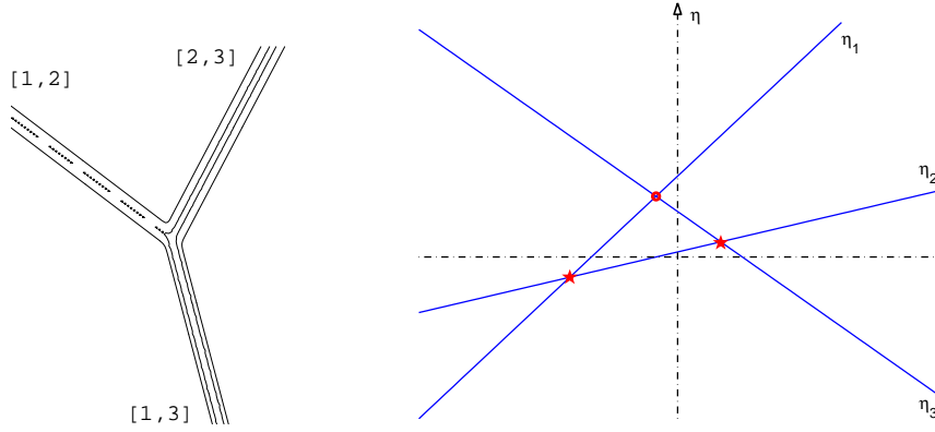
Figure 4. The Y-shape graph (left) illustrating a fundamental resonance with (k_1, k_2, k_3) = (-1, -\frac{1}{4}, \frac{3}{4}) and the corresponding functions \eta_i(c) , i = 1, 2, 3 (right). The graph to the left represents contour lines of u(x, y, t) . The circle at the level set I(0) corresponds to the incoming soliton, and the stars at I(1) correspond to the outgoing solitons.
