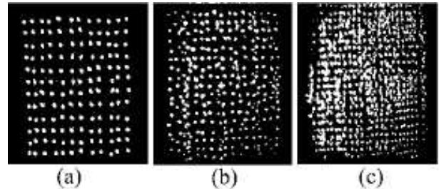
FIG. 2: Determining critical separation in a rectangular lattice, after 20 mm propagation. (a) Above-critical 12 x 12 array with \Delta x = 70\mu\text{m} , \Delta y = 85\mu\text{m} . (b) Slightly below-critical 17 x 17 array with \Delta x = 60\mu\text{m} , \Delta y = 75\mu\text{m} . (c) Below-critical 25 x 25 array with \Delta x = 50\mu\text{m} , \Delta y = 65\mu\text{m} .
