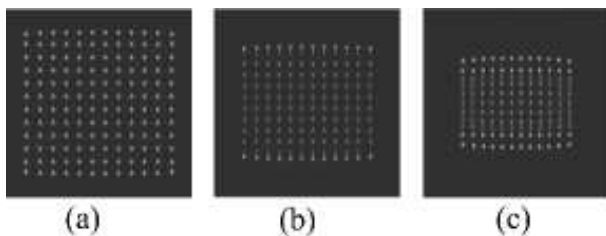
FIG. 3: Quadratic 12 x 12 in-phase solitonic lattice after 35 mm propagation, numerical. Electrooptic coefficient 210 pm/V, external electric field 900 V/cm. The total size of data windows is 1 mm 2 and the initial FWHM size of individual beams 20 μm. (a) \Delta x = \Delta y = 70\mu\text{m} . (b) \Delta x = \Delta y = 60\mu\text{m} . (c) \Delta x = \Delta y = 50\mu\text{m} .
