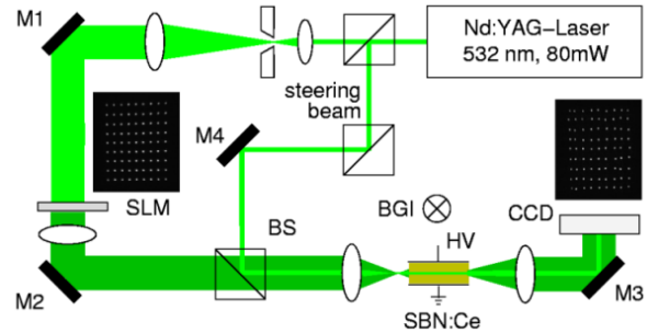
FIG. 1: Experimental setup for the creation of solitonic lattices and control of individual pixels. Insets: typical input and output arrays.
