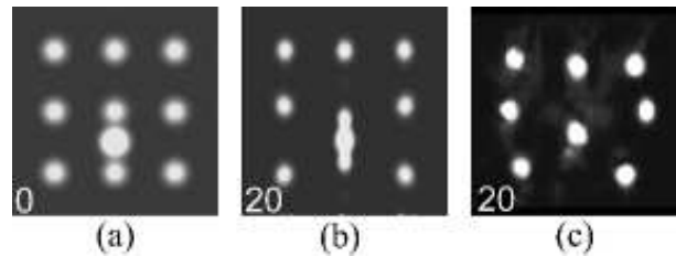
FIG. 6: Comparing numerical and experimental action of a control beam, placed mid-way between two pixels. (a) Initial configuration. (b) Numerical situation after 20 mm propagation. (c) The corresponding experimental situation. The data are 70 \mu\text{m} pixel separation, each spot 20 \mu\text{m} in diameter, coherent lattice, incoherent control. The control beam is three times more intense than any of the pixels.
