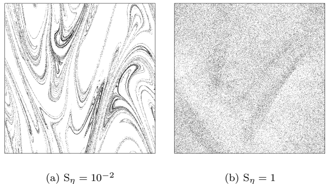
FIG. 2: Snapshots of the position of N = 10^5 heavy particles ( \beta = 0 ) associated to two different Stokes numbers: (a) smaller than the critical value, for which the particles form fractal clusters, and (b) larger than the critical value for which they fill the whole domain. The carrier incompressible flow is generated randomly by 4 independent modes with a finite correlation time.
