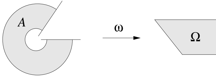
Figure 2: The map \omega : A \rightarrow \Omega .
