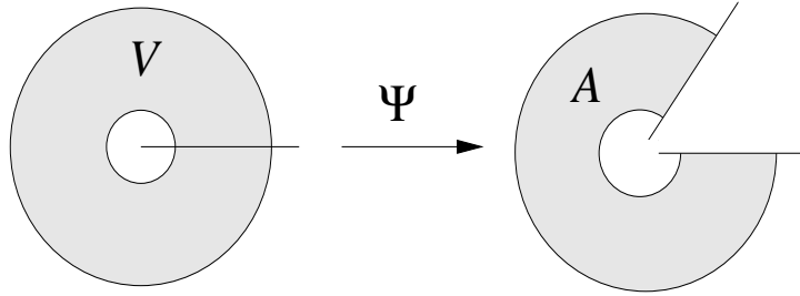
Figure 1: The map \Psi : V_* \rightarrow A .
