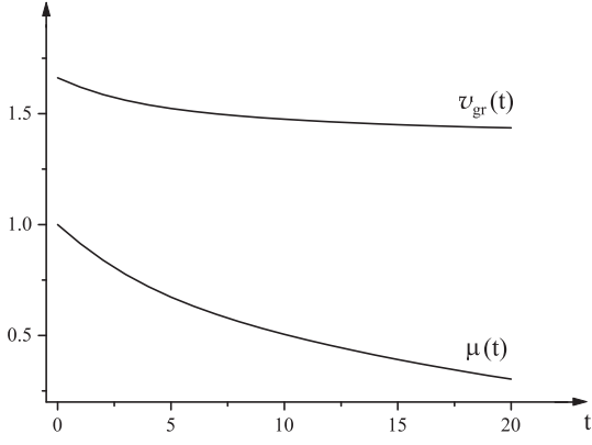
FIG. 2: Evolution of the soliton mass ( m = 2\mu ) and group velocity v_{gr} in the case of linear damping for k = \pi/4 , \epsilon = 0.03 and \mu(t=0) = 1 .
