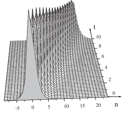
FIG. 3: Evolution of the perturbed AL soliton u_n (8.2) with account for the first-order correction. The soliton parameters are the same as in Fig. 2.
