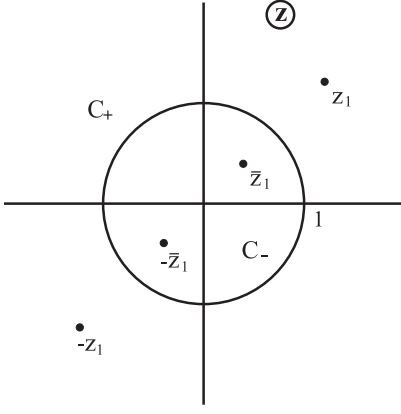
FIG. 1: Typical arrangement of zeros corresponding to a single soliton.
