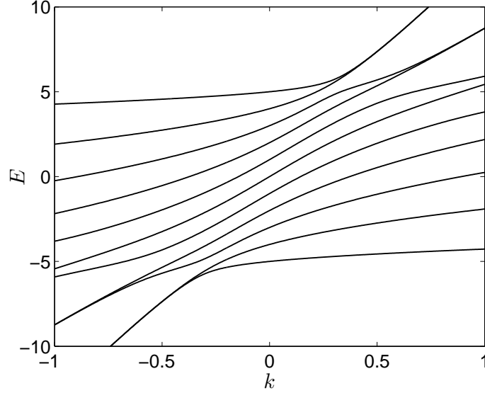
Figure 1. Energy levels E versus coupling k of the Hamiltonian (1) for N = 10 , \mu = 0 , and \mathcal{E} = 1 .
